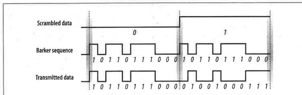
Receivers can look at the number of 1s in a received bit time. The Barker sequence has six 1s and five 0s. An 11-bit sequence with six 1s must therefore correspond to a transmitted 0, and an 11-bit sequence with six 0s must correspond to a transmitted 1. In addition to counting the numbers of 1s and 0s, the receiver can analyze the pattern of received bits to infer the value of the transmitted bit.
