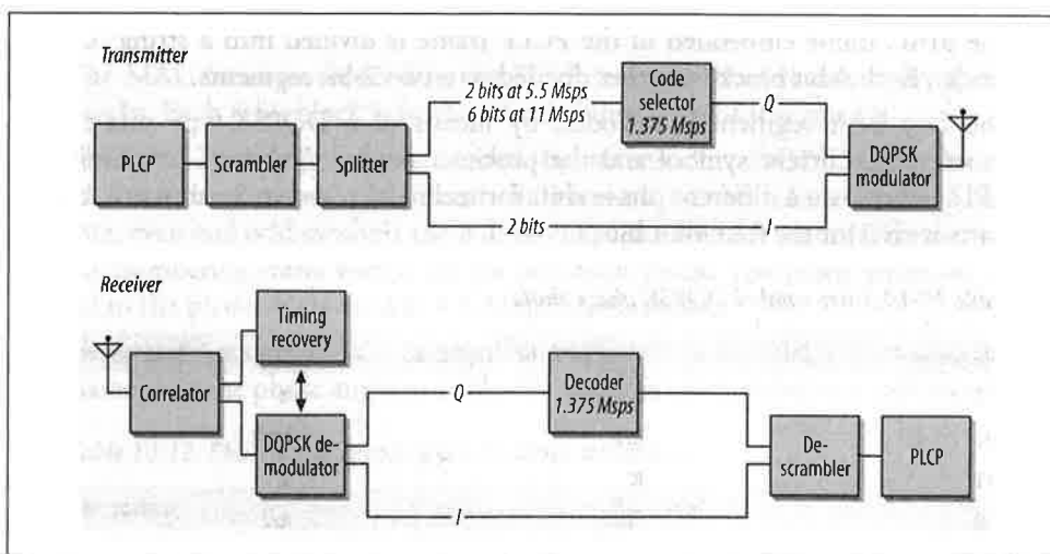
Figure 10-28. HR/DSSS transceiver
