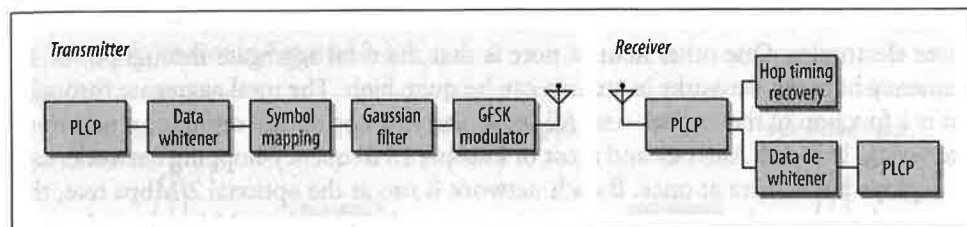
Figure 10-10. Frequency-hopping transceiver
