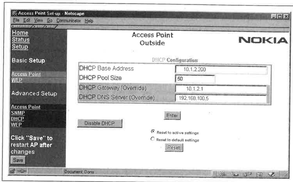
Figure 14-16. DHCP configuration
