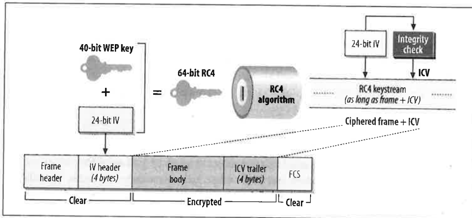
Figure 5-3. WEP operations
