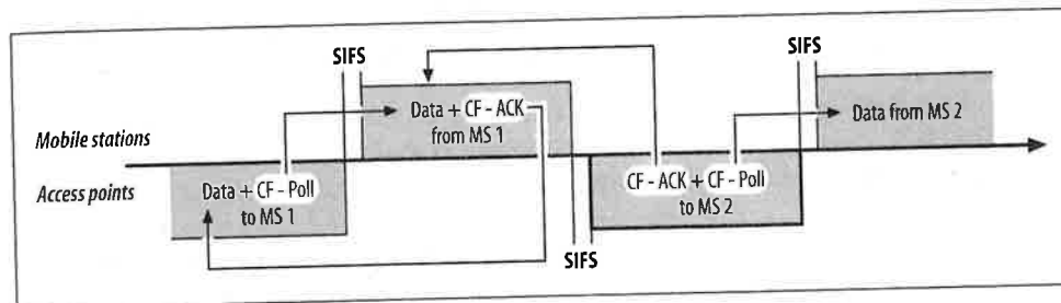
Figure 8-6. CF-Ack+CF-Poll usage
