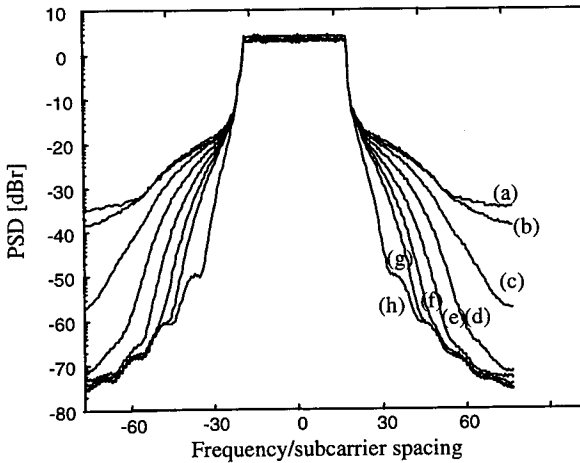
Figure 6.7 Frequency spectrum of an OFDM signal with 32 subcarriers with peak windowing at a threshold level of 3 dB above the rms amplitude. Symbol length is 128 samples (4 times oversampled) and window length is (a) 3, (b) 5, (c) 7, (d) 9, (e) 11, (f) 13, and (g) 15 samples. Curve (h) is the ideal OFDM spectrum.
