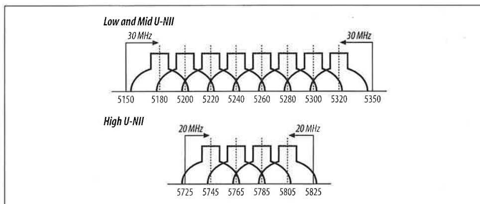
Figure 11-10. Operating bands from Table 11-1
