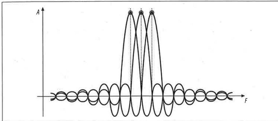
Figure 11-3. Orthogonality in the frequency domain
