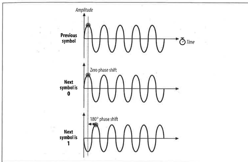
Figure 10-19. DBPSK encoding
