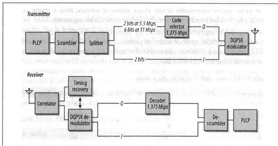
Figure 10-28. HR/DSSS transceiver
