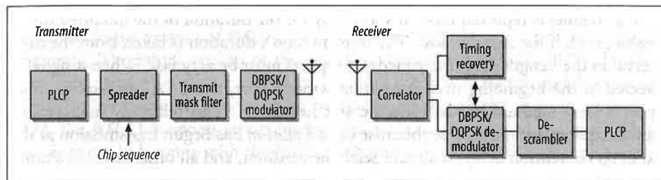
Figure 10-24. Direct-sequence transceiver
