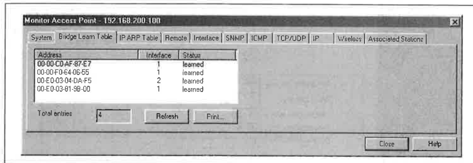
Figure 14-13. Bridge table
