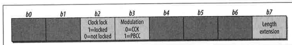
Figure 10-27. Service field in the HR/DSSS PLCP header
