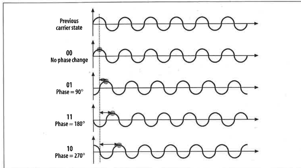
Figure 10-21. DQPSK encoding
