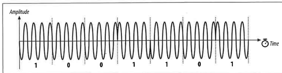
Figure 10-20. The letter M encoded in DBPSK
