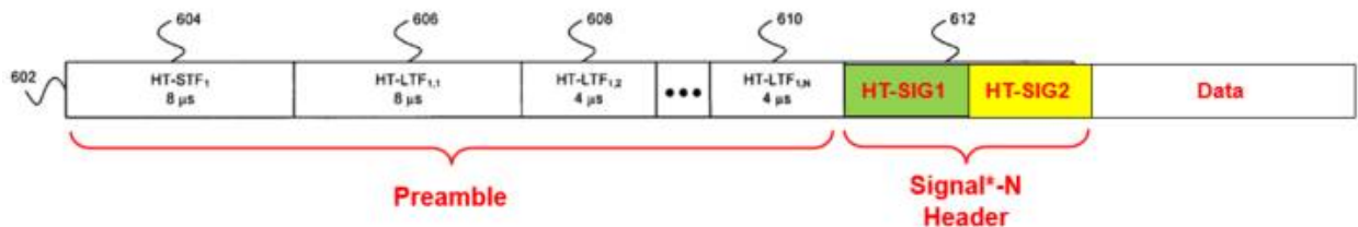
NR Greenfield PPDU (Hansen’s Figure 3a and Excerpt from Figure 6a with Signal*-N symbols)
