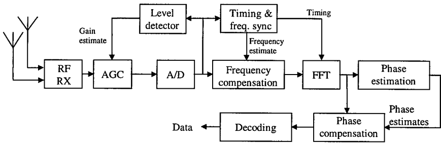
Figure 10.5 OFDM receiver.
