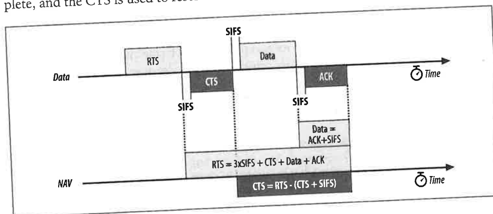
Figure 3-17. RTS/CTS lockout
