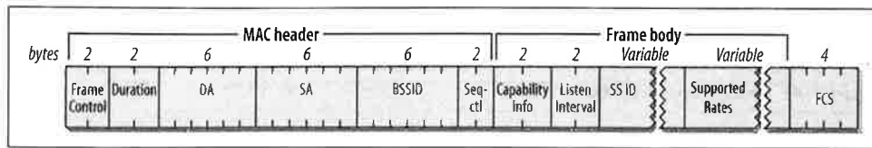
Figure 4-44. Association Request frame
