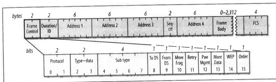
Figure 3-10. Frame control field
