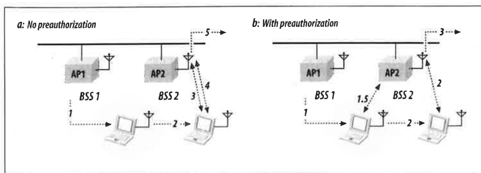
Figure 7-6. Time savings of preauthentication
