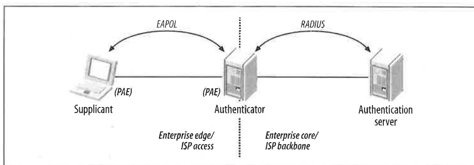
Figure 6-6. 802.1x architecture
