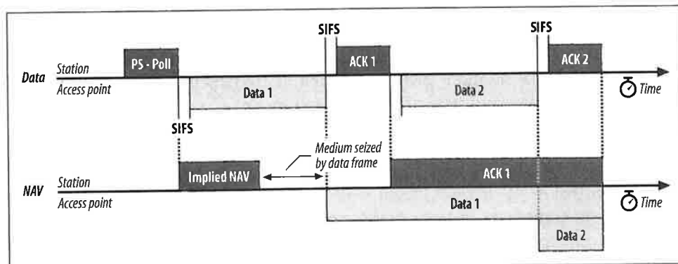
Figure 3-20. Immediate PS-Poll response with fragmentation
