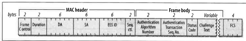
Figure 4-47. Authentication frames
