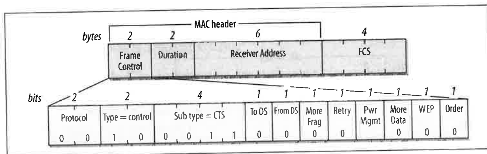
Figure 4-15. CTS frame
