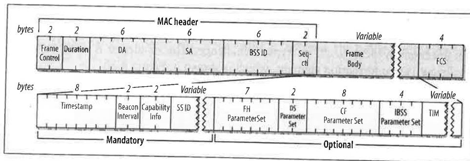
Figure 4-39. Beacon frame
