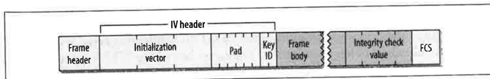
Figure 5-4. WEP frame extensions
