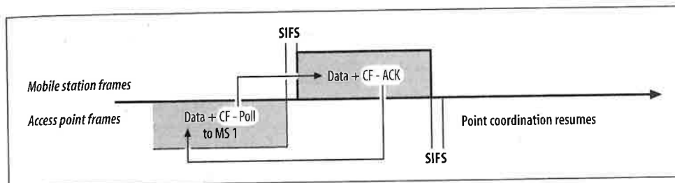
Figure 8-3. Data+CF-Ack usage
