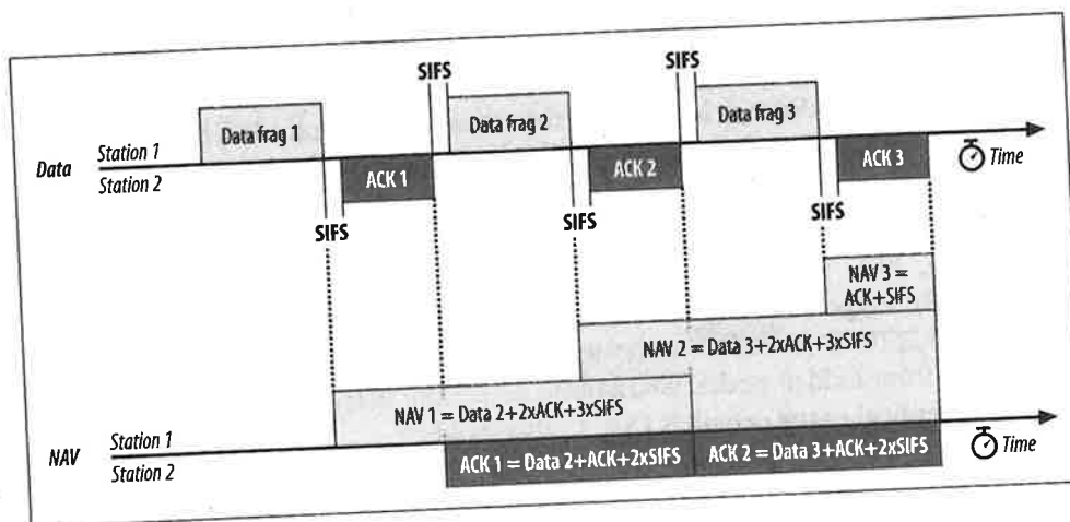
Figure 3-16. Fragmentation
