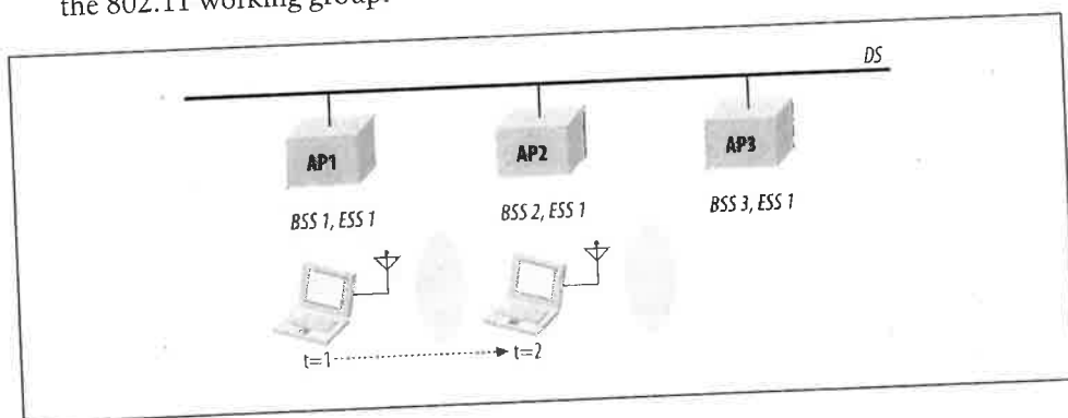
Figure 2-9. BSS transition
