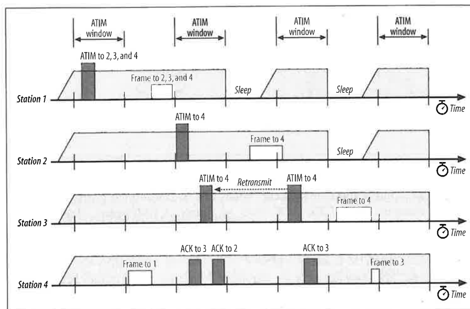
Figure 7-16. Effect of ATIM on power-saving modes in an IBSS network
