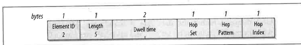
Figure 4-34. FH Parameter Set information element
