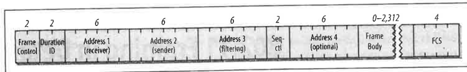
Figure 4-1. Generic data frame
