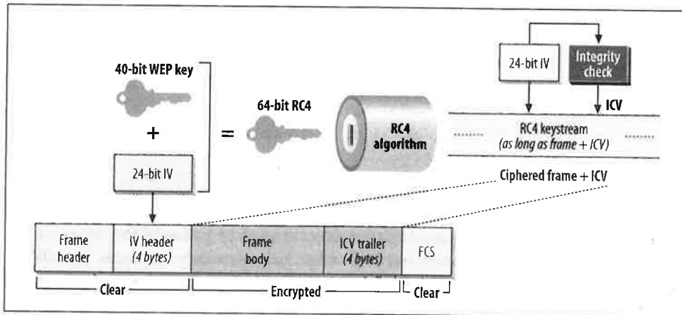
Figure 5-3. WEP operations
