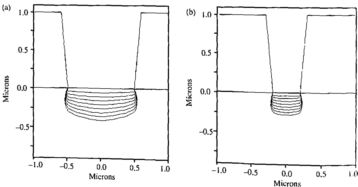
Figure 10-29 SPEEDIE simulations for etching of Si with the linear etch model illustrating Aspect Ratio Dependent Etching (ARDE). Physical-only etching (with arrival angle distribution factor n = 10 ) is done for two different mask opening widths: (a) mask opening = 1\text{ }\mu\text{m} ; (b) mask opening = 0.4\text{ }\mu\text{m} . Deeper etching occurs for the wider mask opening.
