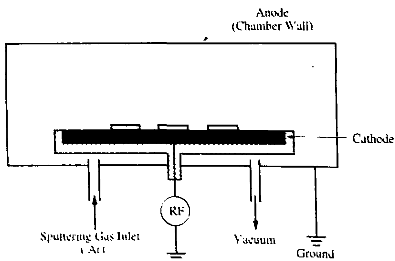
Figure 10-17 Illustration of sputter etch system.
