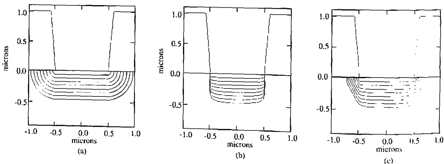
Figure 10-27 SPEEDIE simulations for etching of Si with linear etch model: (a) all chemical etching, showing isotropic etching; (b) all physical or ionic etching, showing very anisotropic etching; (c) half-chemical, half-ionic etching, showing a combination of isotropic and anisotropic etching. The different curves correspond to different times in the etch simulation.
