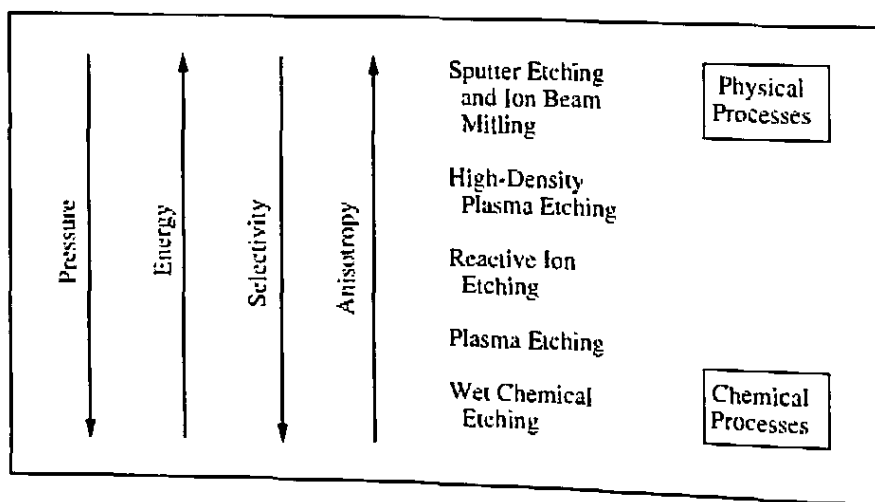
Figure 10-19 Summary of trends of different etch systems.
