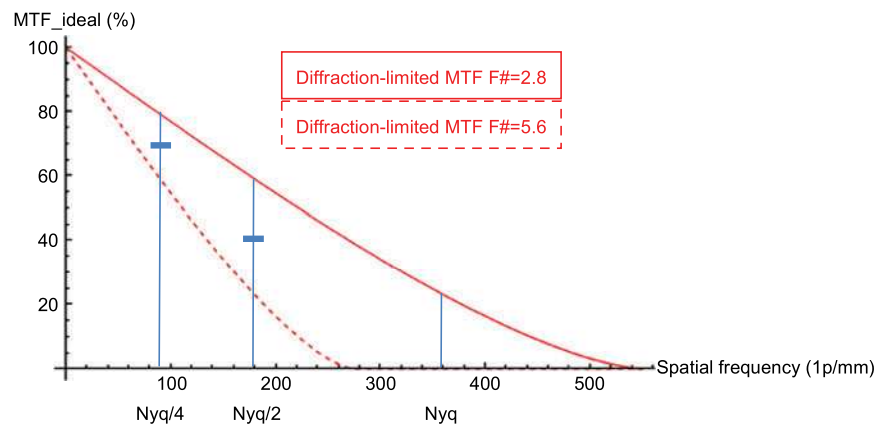
Figure 3 MTF of diffraction-limited lens at F\#=2.8 (solid line) and F\#=5.6 (dashed line) compared to the contrast requirements at the center of field of >70\% at 90 \text{ lp/mm} (Nyquist/4) and >40\% at 180 \text{ lp/mm} (Nyquist/2).
