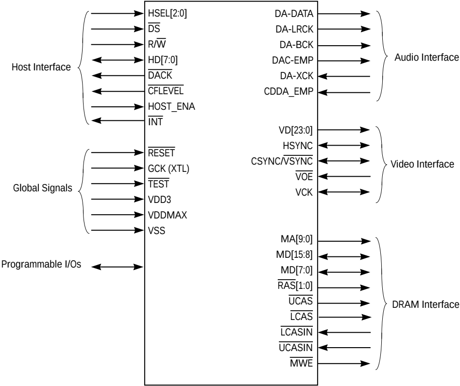
Figure 8-2 CL480PC, External Interface Signals
