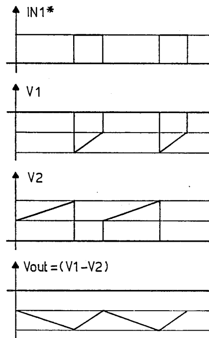
FIG. 3 (prior art)
