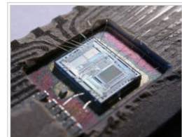
The integrated circuit from an Intel 8742, an 8-bit microcontroller that includes a CPU running at 12 MHz, 128 bytes of RAM, 2048 bytes of EPROM, and I/O in the same chip.
