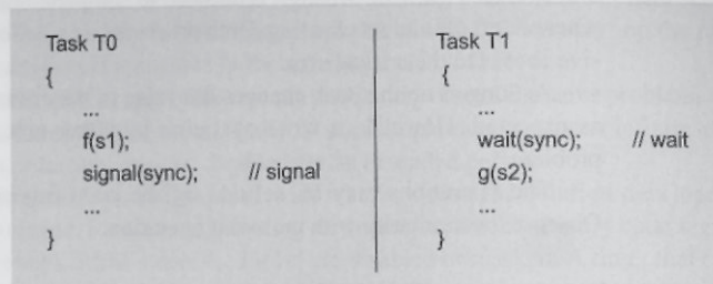
Figure 12.37 Using a Semaphore to Control the Order of Execution
