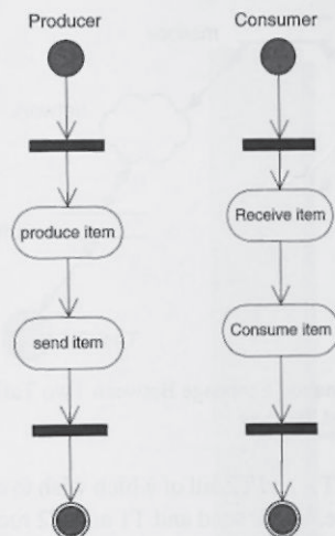
Figure 12.18 Activity Diagram Illustrating a Producer-Consumer Exchange
