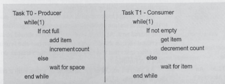
Figure 12.28 Pseudo-Code Modeling a Producer–Consumer Information Exchange
