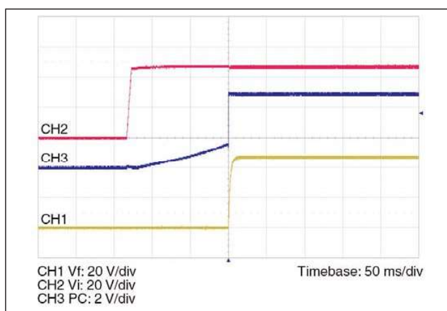
Figure 2 — Vf and PC response from power up
