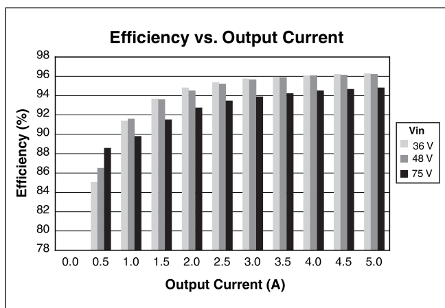
Figure 6 — Efficiency vs. output current at 48 Vf
