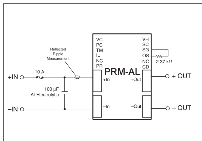
Figure 5 — Input filter capacitor recommendation
