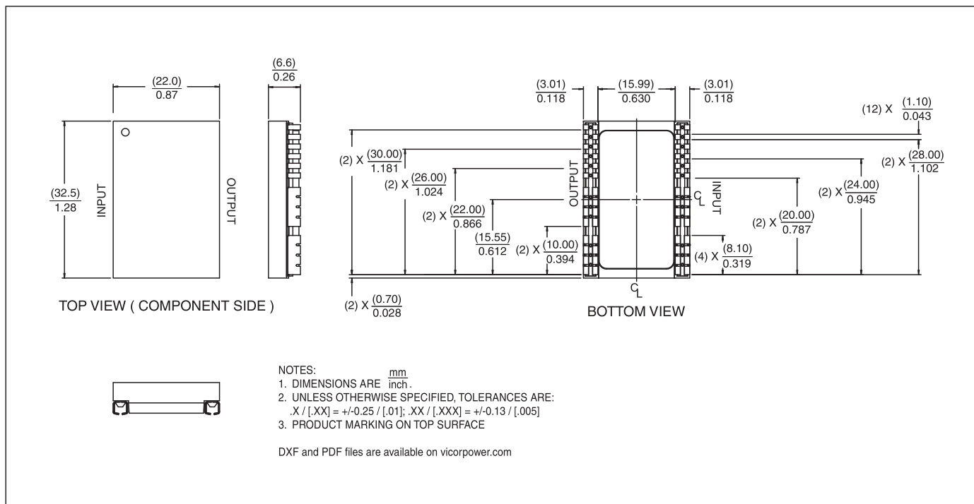
Figure 19—PRM J-Lead mechanical outline
