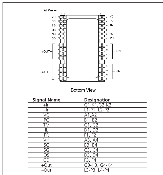
Figure 15 — PRM pin configuration
