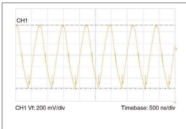
Figure 13 — Output ripple full load no bypass capacitance
