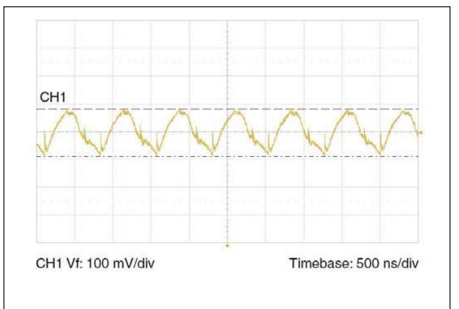
Figure 14 — Output ripple full load 10μF bypass capacitance
