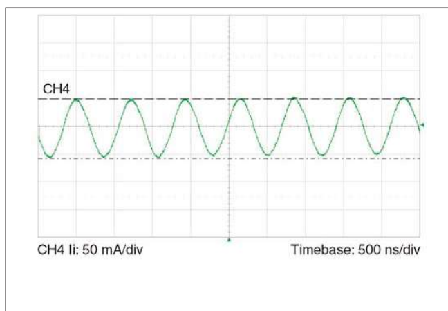
Figure 4 — Input reflected ripple current
