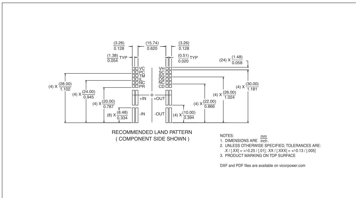
Figure 20— PRM J-Lead PCB land layout information
