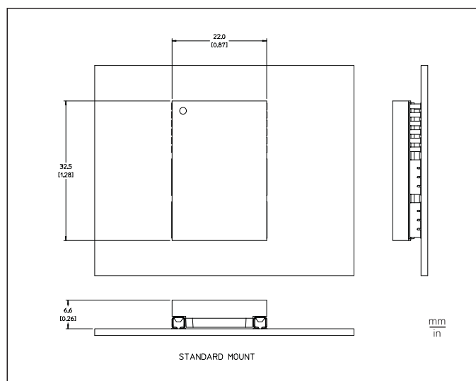
Figure 21 — Standard mounting – package F
