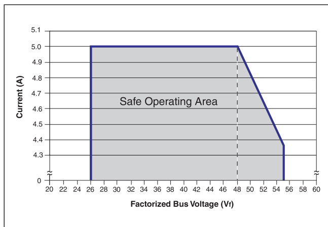
Figure 17 — P048K048T24AL rating based on Factorized Bus voltage
