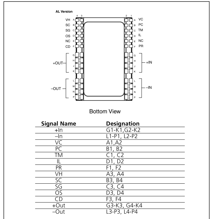
Figure 15 — PRM pin configuration
