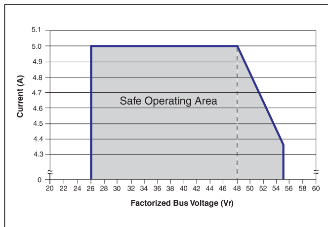
Figure 17 — P048F048T24AL rating based on Factorized Bus voltage
