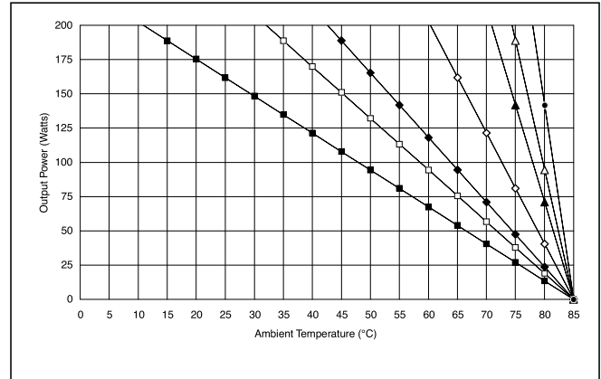
Figure 21-38 — 1-Up FlatPAC 12 – 48 V output
