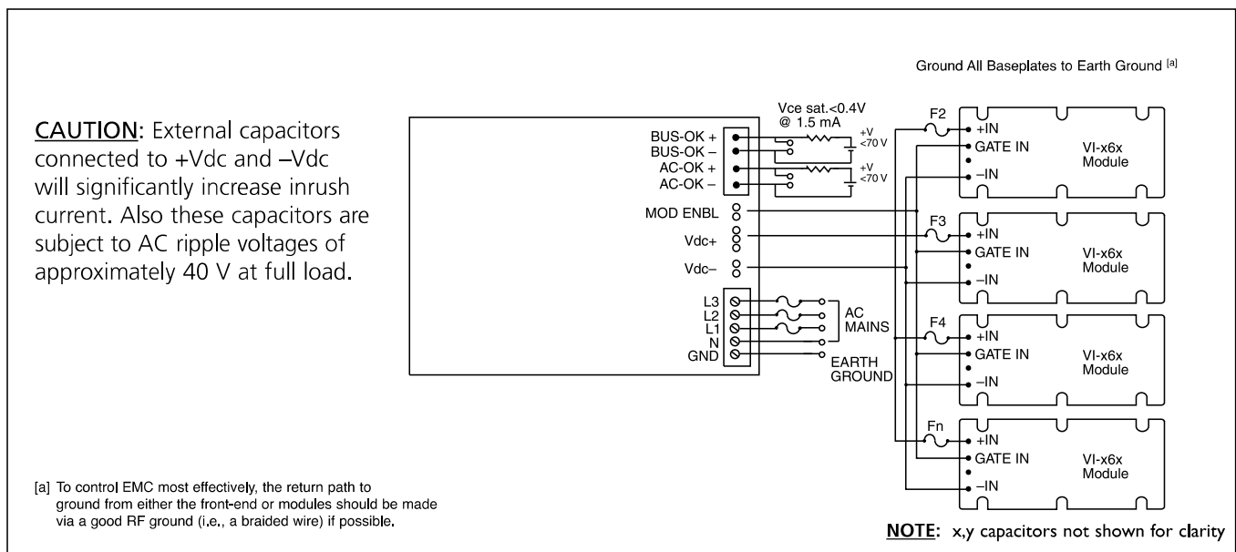
Figure 16-4 — 5.0 kW Front-end
