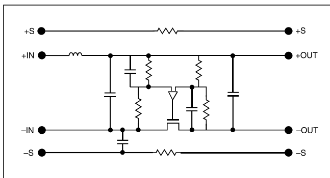
Figure 15–2 — Basic RAM schematic
