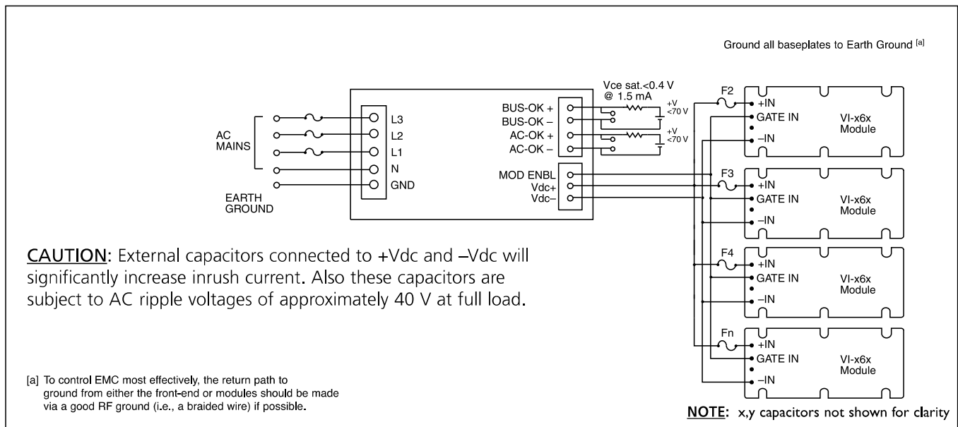
Figure 16-3 — 1.5, 3.0 kW Front-end
