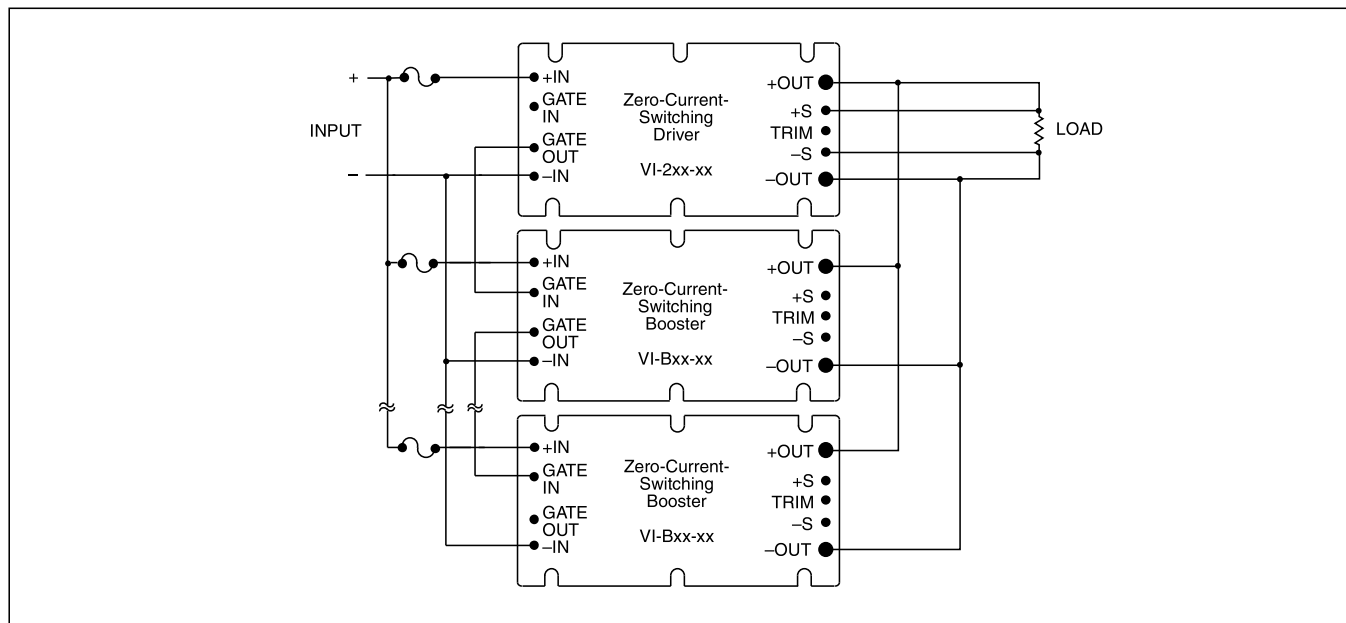
Figure 8-1 — Parallel array
