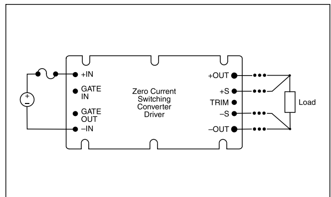
Figure 7–4 — Remote sensing
