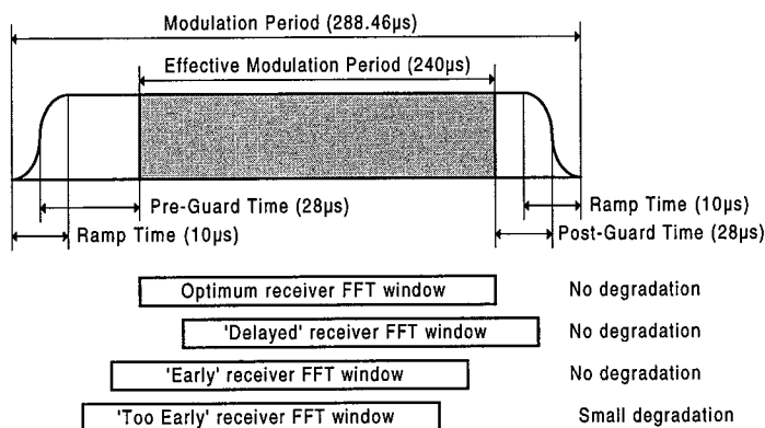
Figure 9.9 OFDMA burst and synchronization requirements.
