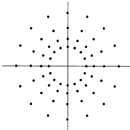
Figure 5.14 64-DAPSK constellation.
