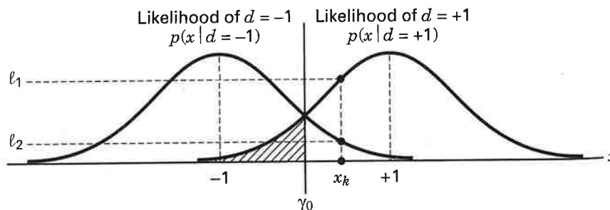
Figure 8.20 Likelihood functions.
