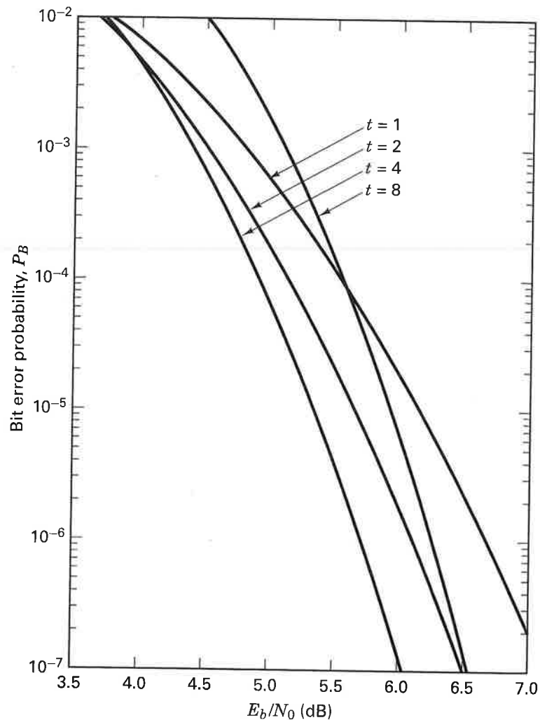
Figure 8.2 Bit error probability versus E_b/N_0 performance of several n = 31 , t -error correcting Reed-Solomon coding systems with 32-ary MFSK modulation over an AWGN channel. (Reprinted with permission from Data Communications, Networks, and Systems , ed. Thomas C. Bartee, Howard W. Sams Company, Indianapolis, Ind., 1985, p. 312. Originally published in J. P. Odenwalder, Error Control Coding Handbook , M/A-COM LINKABIT, Inc. San Diego, Calif., July 15, 1976, p. 92.)
