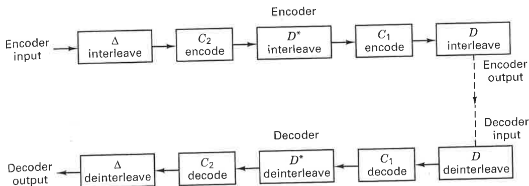
Figure 8.15 CIRC encoder and decoder.
