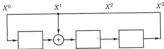
Figure 8.8 Extension field elements can be represented by the contents of a binary linear feedback shift register (LFSR) formed from a primitive polynomial.
