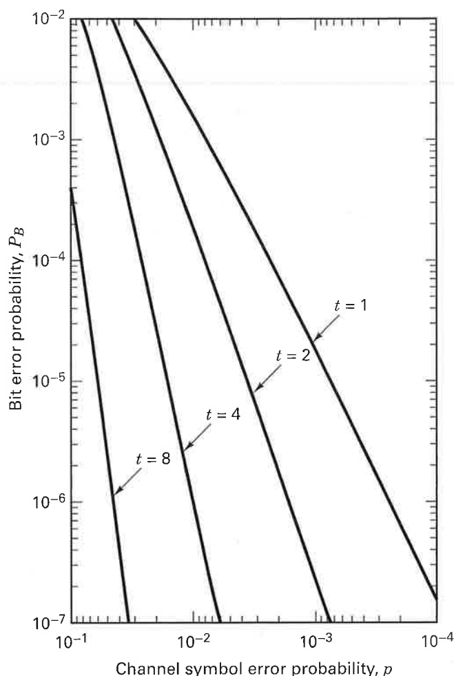
Figure 8.1 P_B versus p for 32-ary orthogonal signaling and n = 31 , t -error-correcting Reed-Solomon coding. (Reprinted with permission from Data Communications, Networks and Systems , ed. Thomas C. Bartee, Howard W. Sams Company, Indianapolis, Ind., 1985, p. 311. Originally published in J. P. Odenwalder, Error Control Coding Handbook , M/A-COM LINKABIT, Inc., San Diego, Calif., July 15, 1976, p. 91.)
