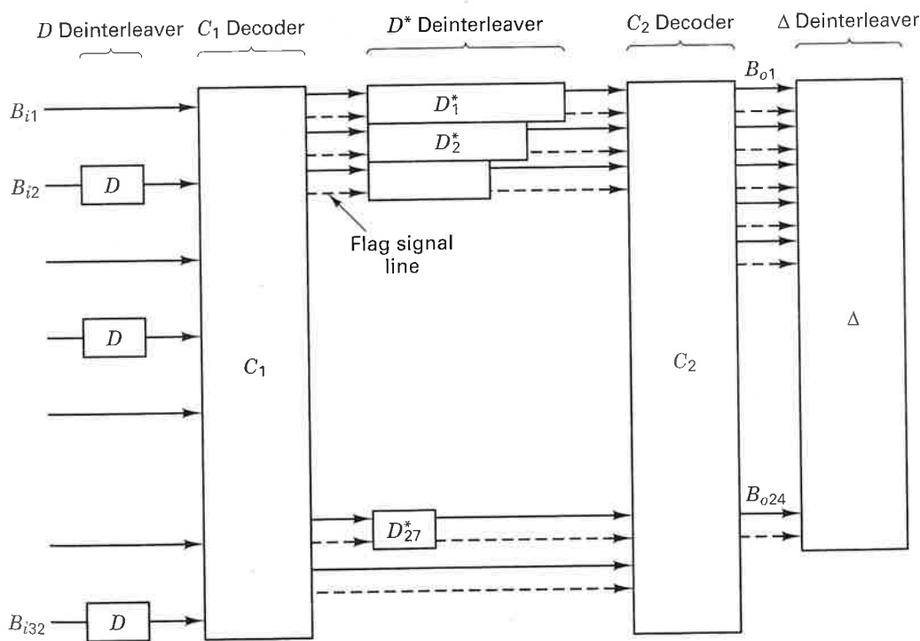
Figure 8.17 Compact disc decoder.
