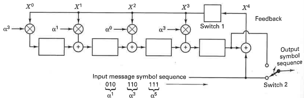
Figure 8.9 LFSR Encoder for a (7,3) R-S code.
