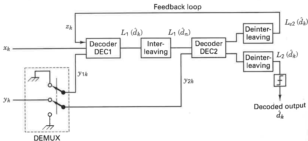
Figure 8.27 Feedback decoder.
