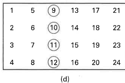
Figure 8.11 Block interleaver example. (a) M \times N block interleaver. (b) Five-symbol error burst. (c) Nine-symbol error burst. (d) Periodic single-error sequence spaced N = 6 symbols apart.
