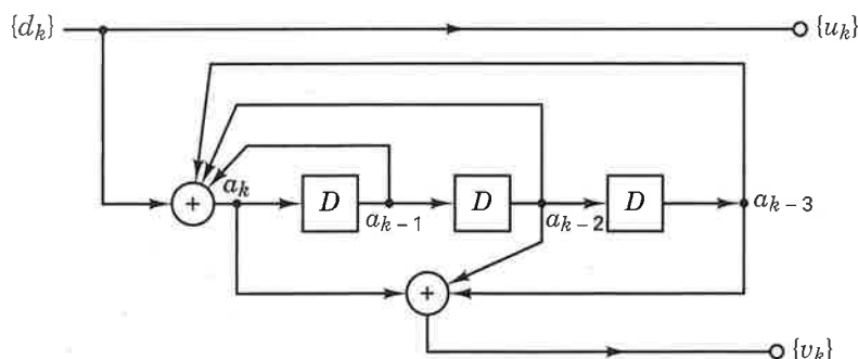
Figure P8.2 Recursive systematic convolutional (RSC) encoder, rate \frac{1}{2} , K = 4 .
