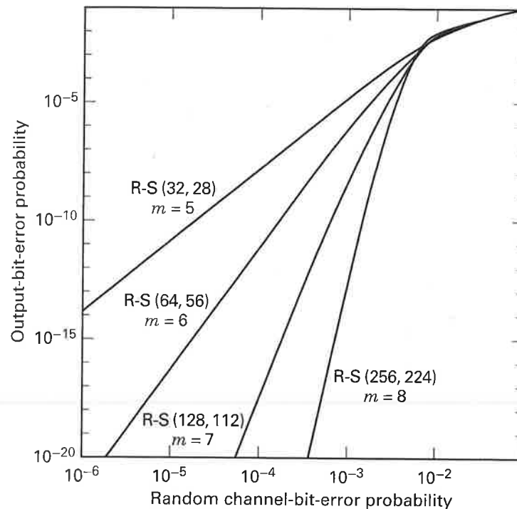
Figure 8.4 Reed-Solomon, rate 7/8, decoder performance as a function of symbol size.
