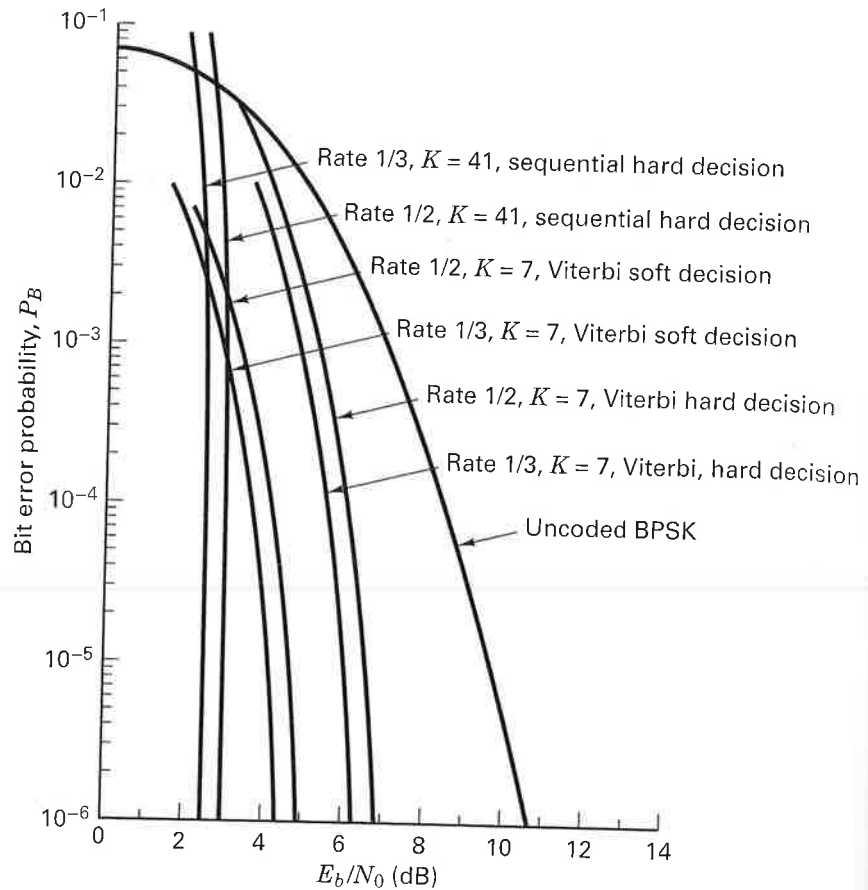
Figure 7.24 Bit error performance for various Viterbi and sequential decoding schemes using coherent BPSK over an AWGN channel. (Reprinted with permission from J. K. Omura and B. K. Levitt, "Coded Error Probability Evaluation for Antijam Communication Systems," IEEE Trans. Commun. , vol. COM30, no. 5, May 1982, Fig. 4, p. 900. © 1982 IEEE.)
