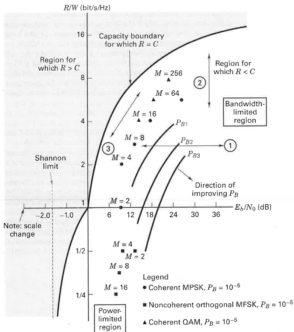
Figure 9.6 Bandwidth-efficiency plane.
