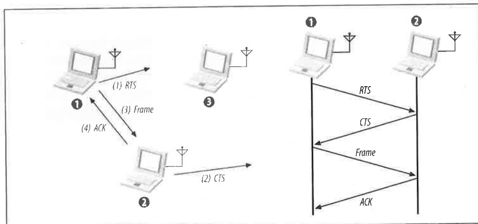
Figure 3-3. RTS/CTS clearing
