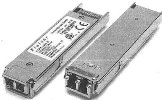
Figure 18-9. Example of XFP device (courtesy of Finisar Corporation)
