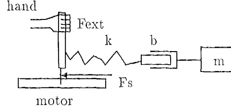
Figure 5: A joystick system
