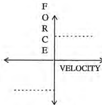
Figure 3-9 Force vs. Velocity for Friction Condition
