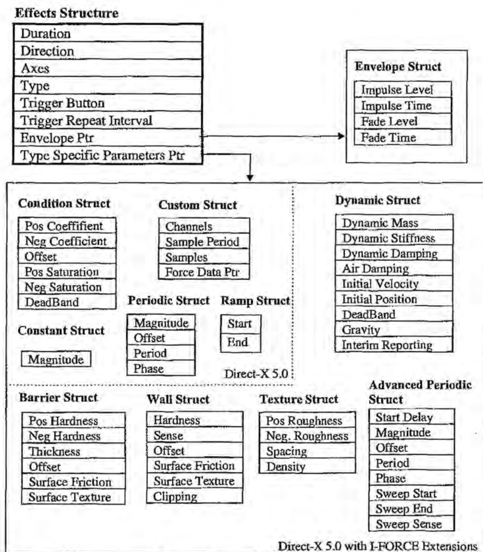
Figure 6-1 Complete Architecture
