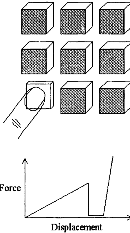
Figure 24: Virtual Buttons and a Typical Force-Displacement Curve
