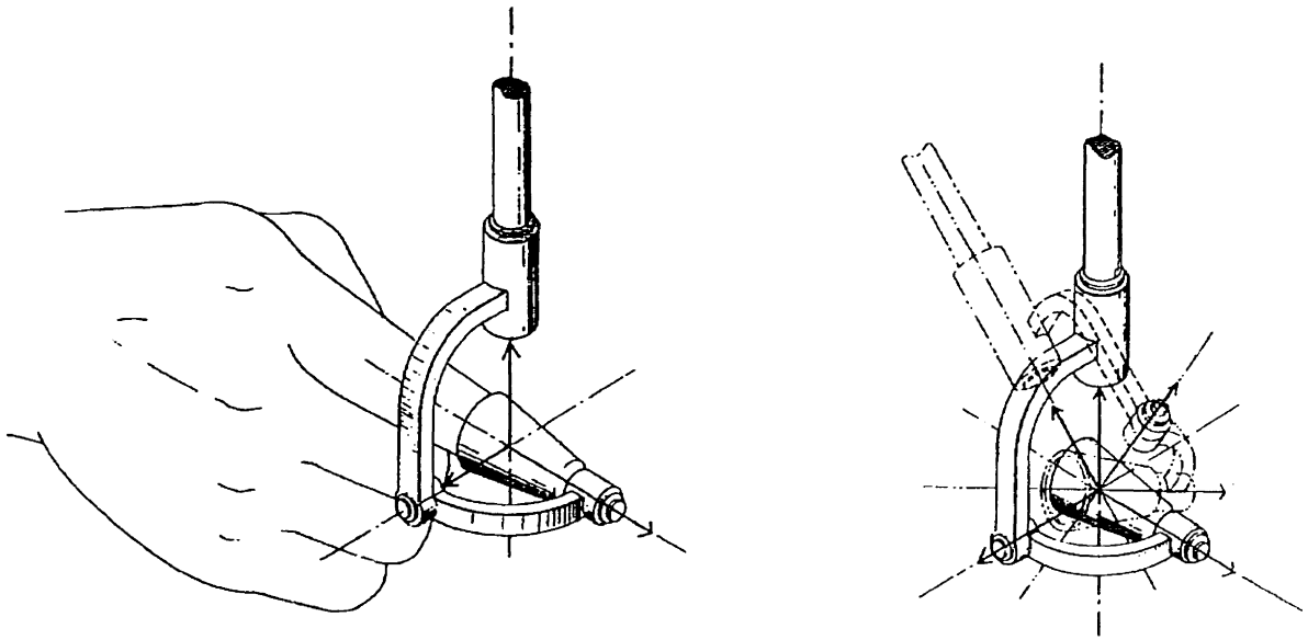
Figure 3: The Thimble-Gimbal
