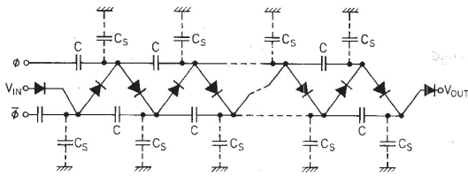
Fig. 1. Basic Cockcroft-Walton voltage multiplier. Usually implemented with discrete components such that C \gg C_S .
