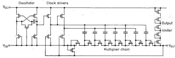
Fig. 5. Practical implementation of multiplier using MOS technology.
