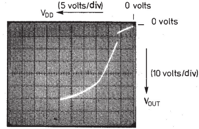
Fig. 7. Voltage characteristics of MOS voltage multiplier driving a 10-M \Omega load.
