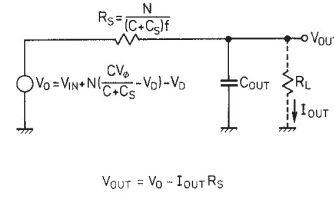
Fig. 4. Equivalent circuit of N -stage multiplier.
