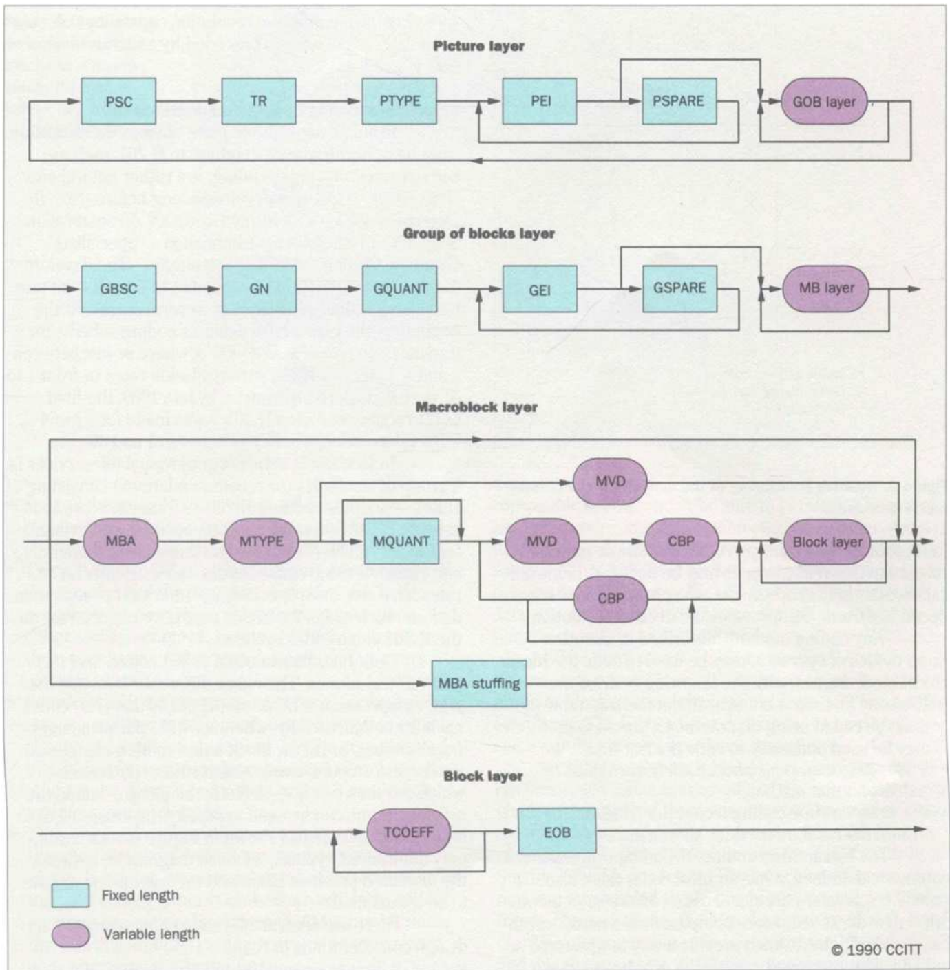
Figure 7. Syntax diagram of the video multiplex coder. 20
