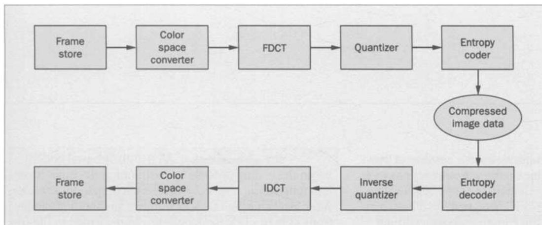
Figure 2. Sequential DCT codec.
