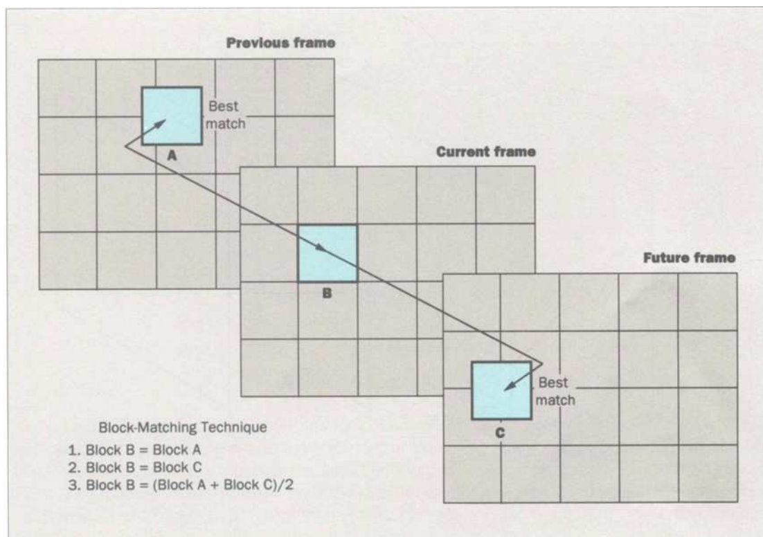
Figure 13. Motion-compensated interpolation.
