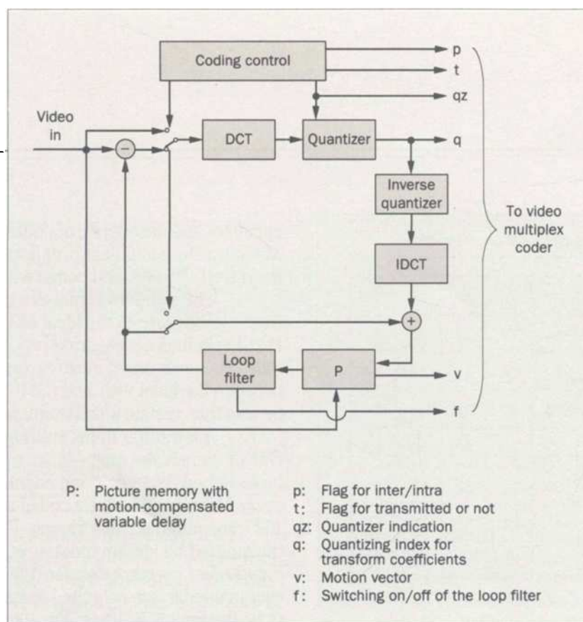
Figure 12. A typical H.261 encoder.
