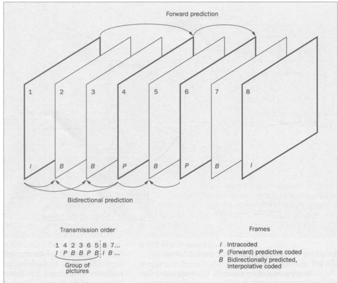
Figure 14. Group of pictures.
