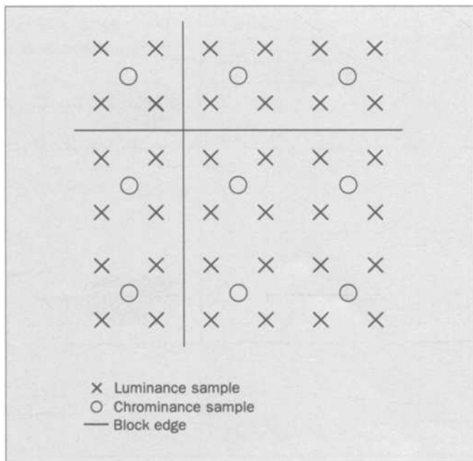
Figure 8. Relative positioning of the luminance and chrominance samples.
