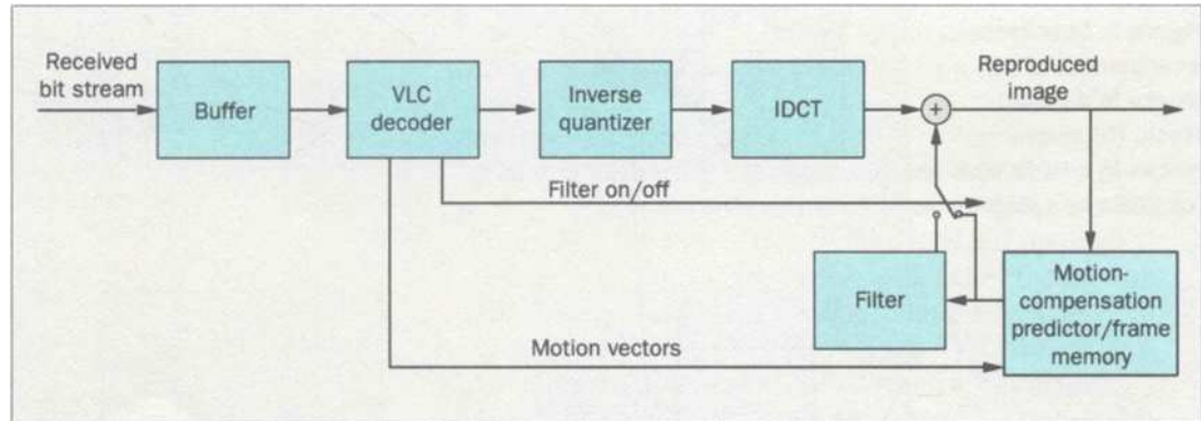
Figure 10. A typical H.261 decoder.
