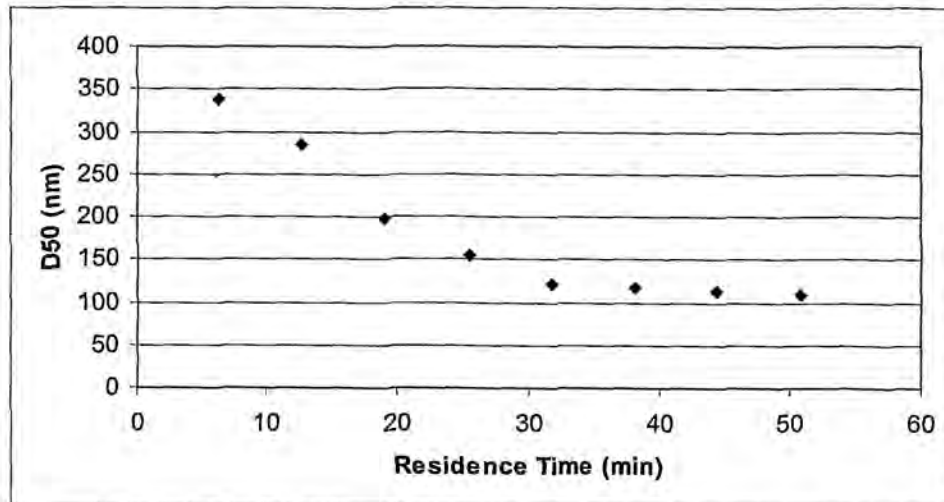
FIGURE 4. Measured D50 values for ganaxolone particles as a function of milling residence time for a typical milling run using a DYNO-Mill KDL equipped with four 64 mm polyurethane agitator discs.
