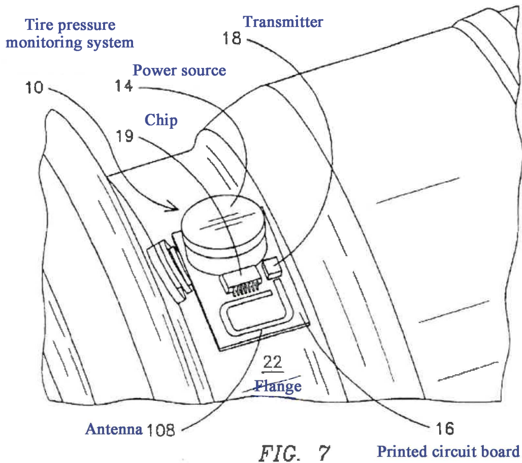
Figure 6 (Figure 7 of Exhibit 11): An exemplary configuration of a direct tire pressure monitoring system (TPMS)
