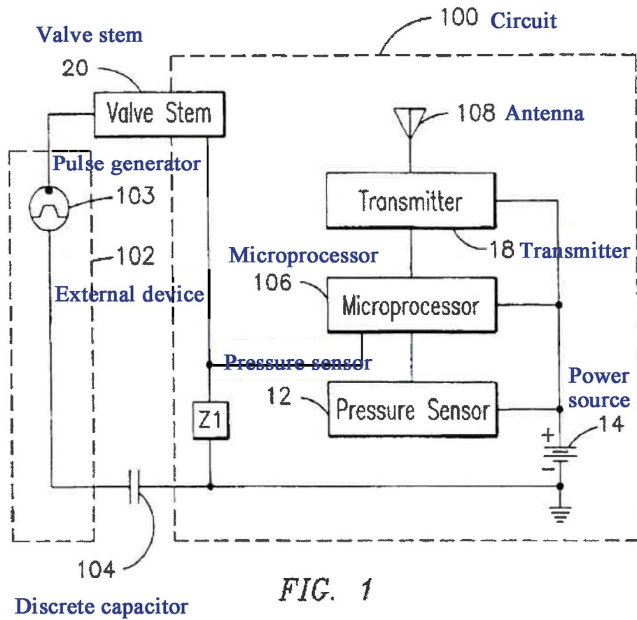
Figure 5 (Figure 1 of Exhibit 11): The schematic diagram of the circuits of various aspects of the present invention
