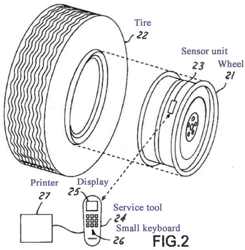
Figure 10 (Figure 2 of Exhibit 8): Tire pressure sensing unit mounted to a wheel and being interrogated by a service tool
