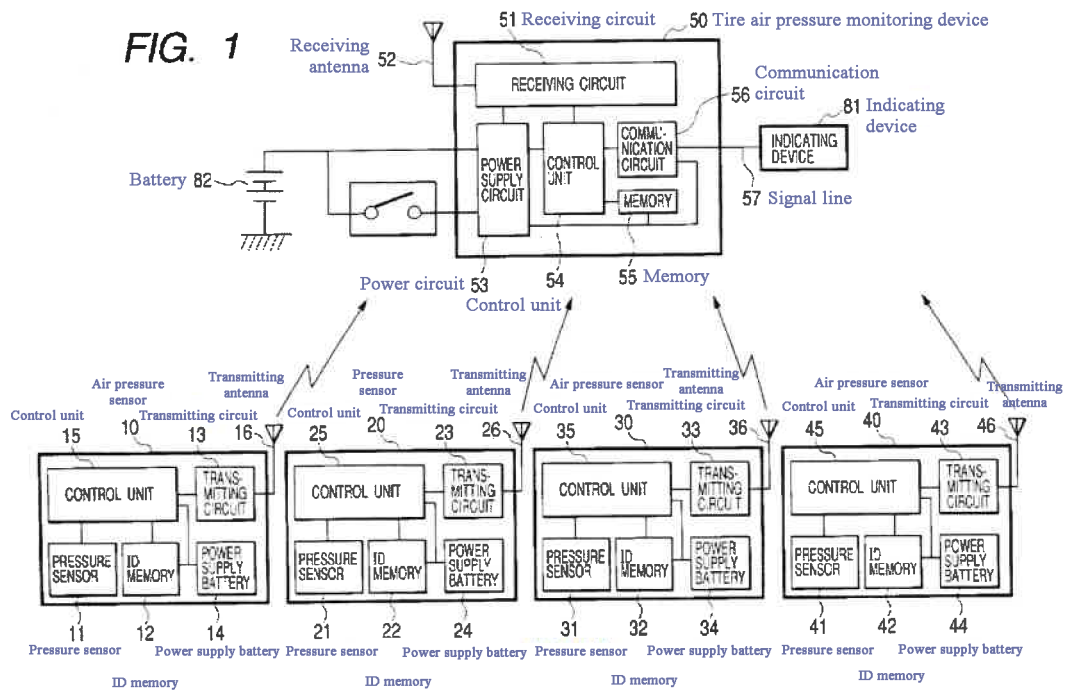
Figure 7 (Figure 1 of Exhibit 12): A block diagram showing the structure of a tire air pressure monitoring system of the first embodiment.
