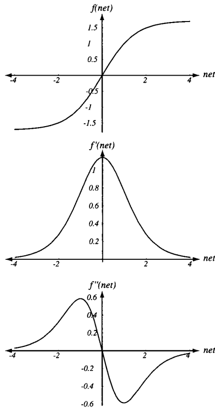
FIGURE 6.14. A useful activation function f(\text{net}) is an anti-symmetric sigmoid. For the parameters given in the text, f(\text{net}) is nearly linear in the range -1 < \text{net} < +1 and its second derivative, f''(\text{net}) , has extrema near \text{net} \simeq \pm 2 .
