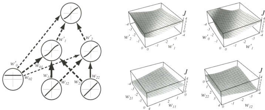
FIGURE 6.9. Two-dimensional slices through the nine-dimensional error surface after extensive training for a 2-2-1 network solving the XOR problem.
