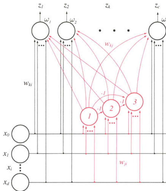
FIGURE 6.26. The training of a multilayer network via cascade-correlation begins with the input layer fully connected to the output layer (black). Such weights, w_{ki} , are fully trained using an LMS criterion, as discussed in Chapter 5. If the resulting training error is not sufficiently low, a first hidden unit (labeled 1, in red) is introduced, fully interconnected from the input layer and to the output layer. These new red weights are fully trained, while the previous (black) ones are held fixed. If the resulting training error is still not sufficiently low, a second hidden unit (labeled 2) is likewise introduced, fully interconnected; it also receives a the output from each previous hidden unit, multiplied by -1 . Training proceeds in this way, training successive hidden units until the training error is acceptably low.
