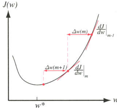
FIGURE 6.21. The quickprop weight update takes the error derivatives at two points separated by a known amount, and by Eq. 53 computes the next weight value. If the error can be fully expressed as a second-order function, then the weight update leads to the weight ( w^* ) leading to minimum error.
