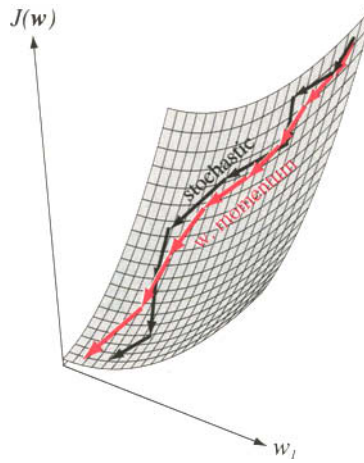
FIGURE 6.18. The incorporation of momentum into stochastic gradient descent by Eq. 37 (red arrows) reduces the variation in overall gradient directions and speeds learning.
