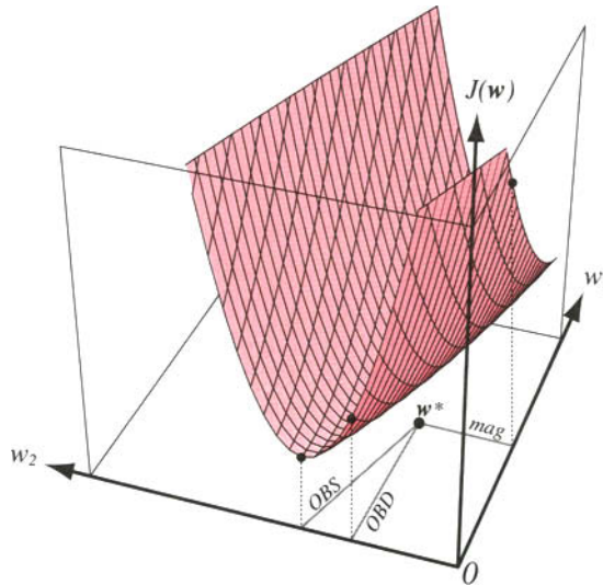
FIGURE 6.28. The figure shows a quadratic error surface as a function of weights, J(\mathbf{w}) , and the global minimum at \mathbf{w}^* . In the second-order approximation to the criterion function, Optimal Brain Damage assumes the Hessian matrix is diagonal, while Optimal Brain Surgeon uses the full Hessian matrix.
