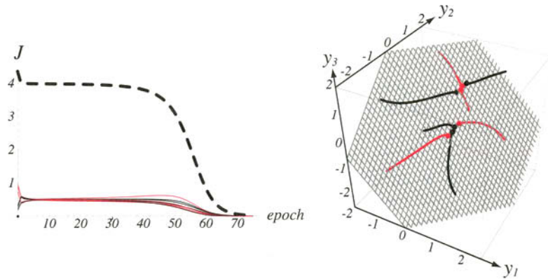
FIGURE 6.11. A 3-3-1 backpropagation network with bias can indeed solve the three-bit parity problem. The representation of the eight patterns at the hidden units ( y_1 y_2 y_3 -space) as the system learns and the planar decision boundary found by the hidden-to-output weights at the end of learning. The patterns of the two classes are indeed separated by this plane, as desired. The learning curve shows the error on individual patterns and the total error J as a function of epoch.
