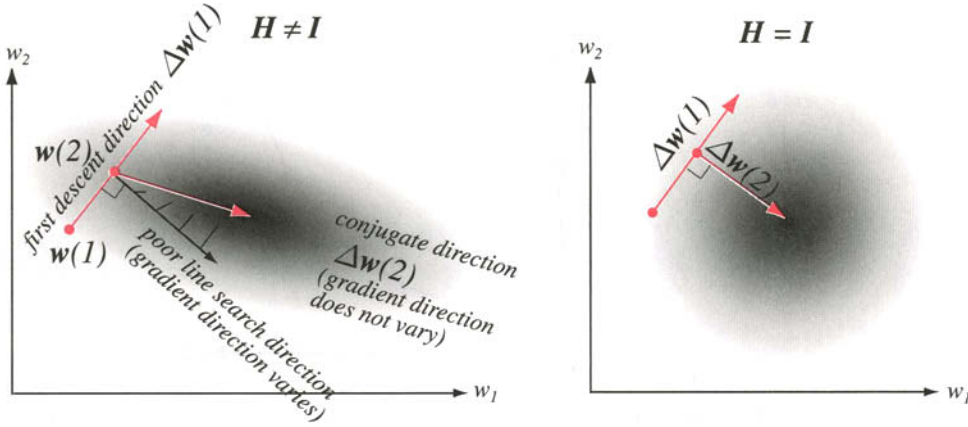
FIGURE 6.22. Conjugate gradient descent in weight space employs a sequence of line searches. If \Delta \mathbf{w}(1) is the first descent direction, the second direction obeys \Delta \mathbf{w}^t(1) \mathbf{H} \Delta \mathbf{w}(2) = 0 . Note especially that along this second descent, the gradient changes only in magnitude, not direction; as such, the second descent does not “spoil” the contribution due to the previous line search. In the case where the Hessian is diagonal (right), the directions of the line searches are orthogonal.
