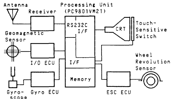
Fig.2 Block diagram of in-vehicle system
