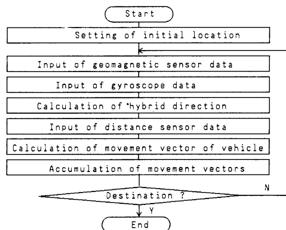
Fig.5 Flowchart of dead reckoning
