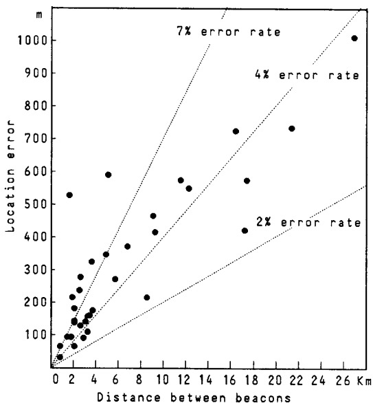
Fig.13 Relationship between navigation error and distance interval
