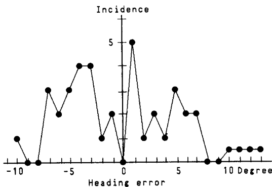
Fig.14 Heading error at beacon points
