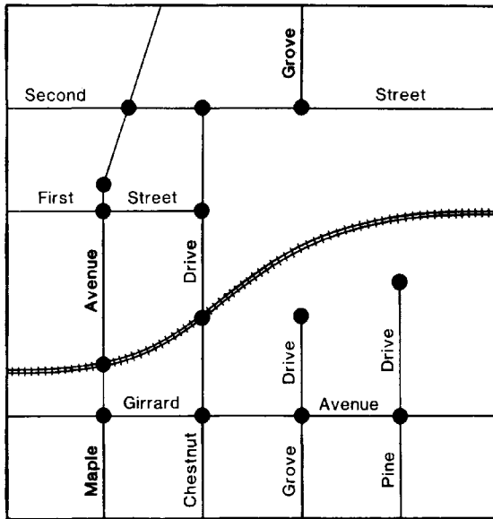
FIGURE 7. Graphic elements of a DIME file.
