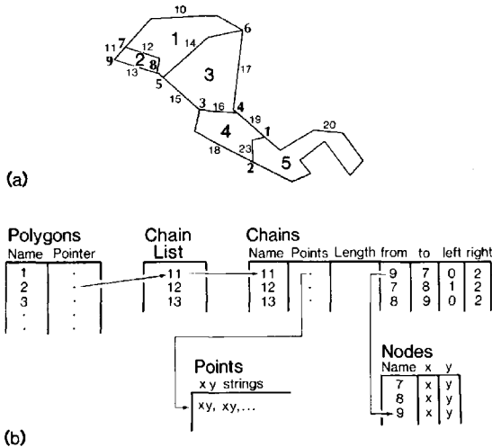
FIGURE 9. a the POLYVRT data model; b the POLYVRT data structure.
