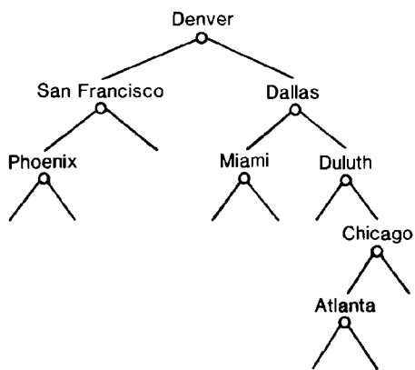
FIGURE 19. The K-d tree data model (from Samet, 1984).
