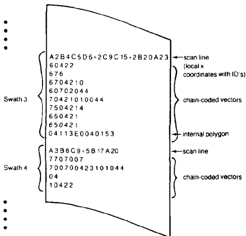
FIGURE 28. Vaster-formatted data in digital form.
