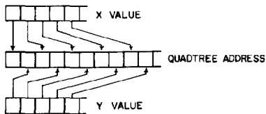
FIGURE 25. Bitwise interlaced indexing scheme.
