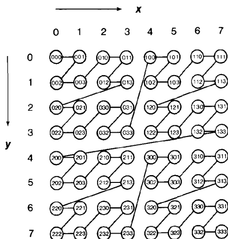
FIGURE 24. The relationship between the morton matrix indexing scheme and the z-shaped Peano curve.
