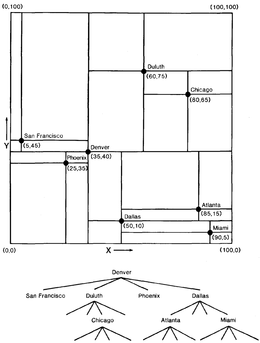
FIGURE 17. The point quadtree data model (from Samet, 1984).
