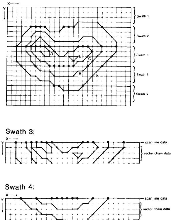
FIGURE 27. a Vaster Organization (logical record-swath); b Individual swaths.
