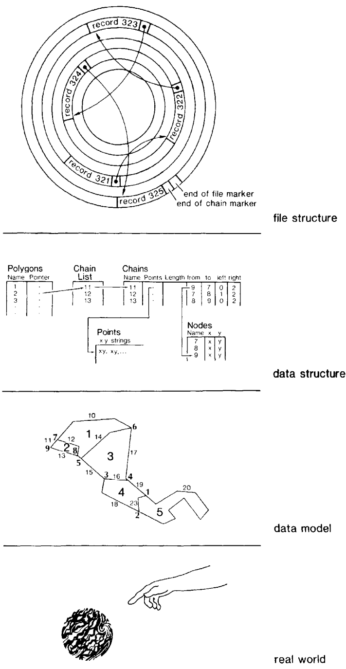
FIGURE 2. Levels of data abstraction.
