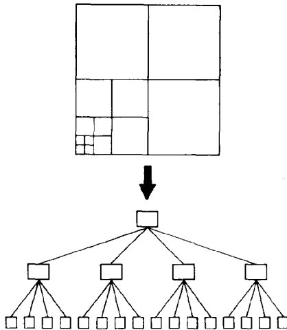
FIGURE 16. The quadtree data model.
