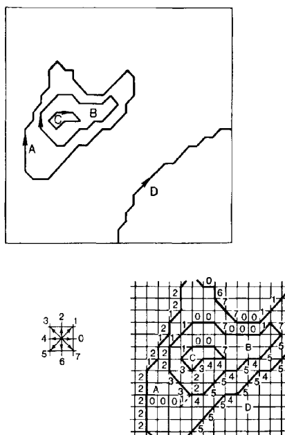
FIGURE 10. Contour map and the resulting chain-coded lines (adapted from Freeman, 1974).
