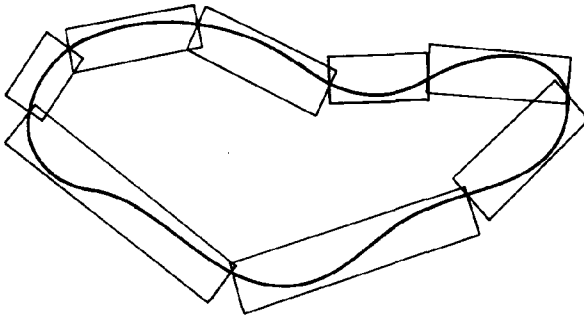
FIGURE 29. The strip tree model.
