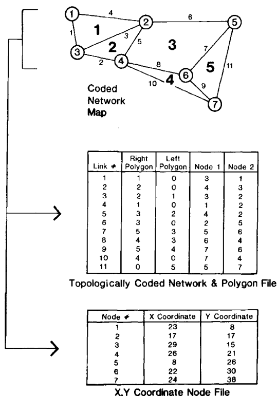
FIGURE 6. The Topological data model (from Dangermond, 1982).
