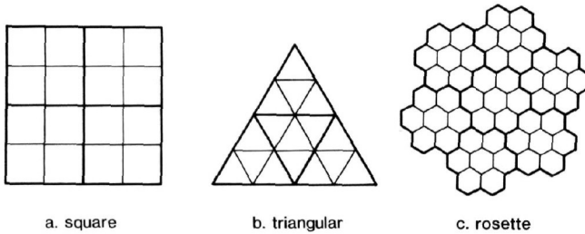
FIGURE 14. The three regular tessellations in recursively subdivided form.
