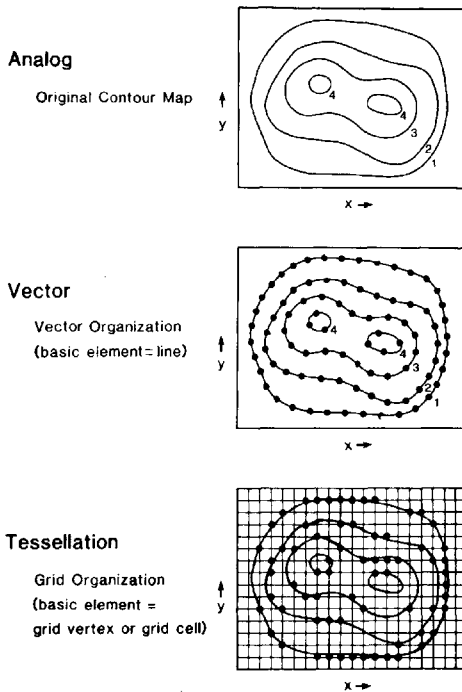
FIGURE 4. Basic types of spatial data models.
