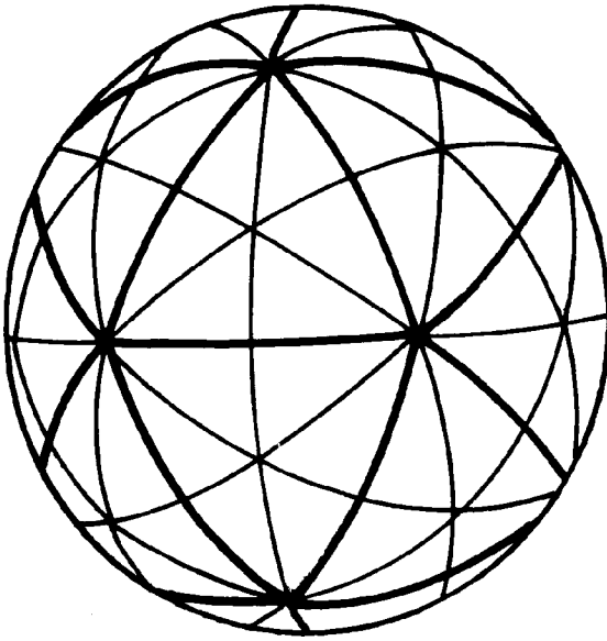
FIGURE 32. Fifteen symmetrically arranged great circles on the sphere.
