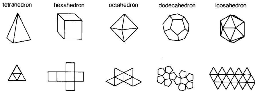
FIGURE 31. The five Platonic solids.
