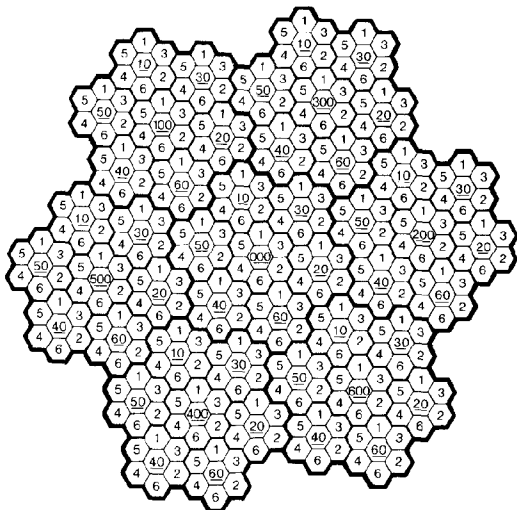
FIGURE 18. A nested hexagonal tessellation with a hierarchical, base 7 indexing scheme.
