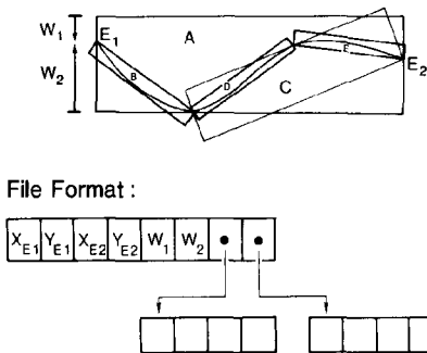
FIGURE 30. Hierarchical structure of strip tree model.
