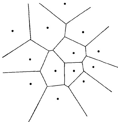
FIGURE 21. An example of Thiessen polygons.
