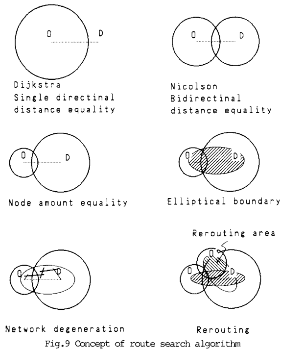
Fig.9 Concept of route search algorithm
