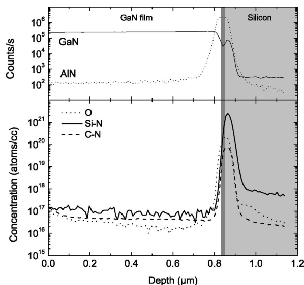
FIG. 4. SIMS results for sample C. The vertical bar indicates the position and the nominal thickness (25 nm) of the AlN layer. Silicon and carbon were detected as species bound to nitrogen.
