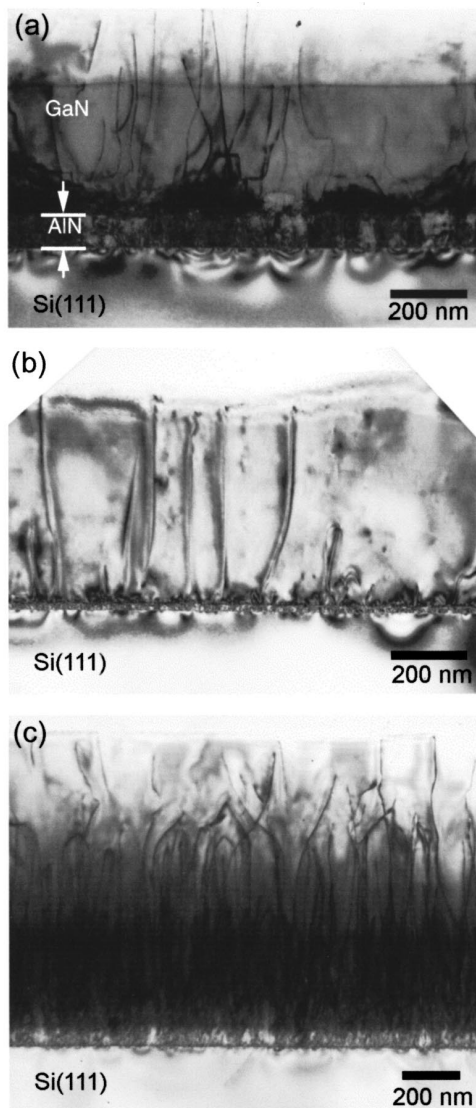
FIG. 1. Transmission electron micrographs of GaN films grown on Si(111) substrates using three buffer schemes (bright field, g = 0002 ). (a) Sample B (the top \sim 200 nm of the GaN film have a different contrast because of shadowing effects during ion milling); (b) sample C; (c) sample E.
