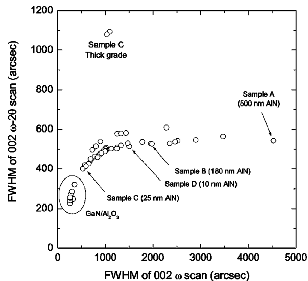
FIG. 2. Typical x-ray diffraction results for GaN/Si(111) samples. Also shown are results for typical GaN films grown on sapphire substrates using a low-temperature GaN nucleation layer.
