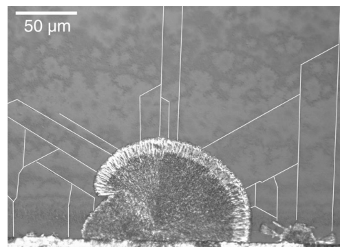
FIG. 3. Optical micrograph showing typical growth defects leading to cracking during the growth of GaN on Si(111) using a thin AlN buffer (sample C). The cracks have been emphasized for clarity. The wafer edge is at the bottom.
