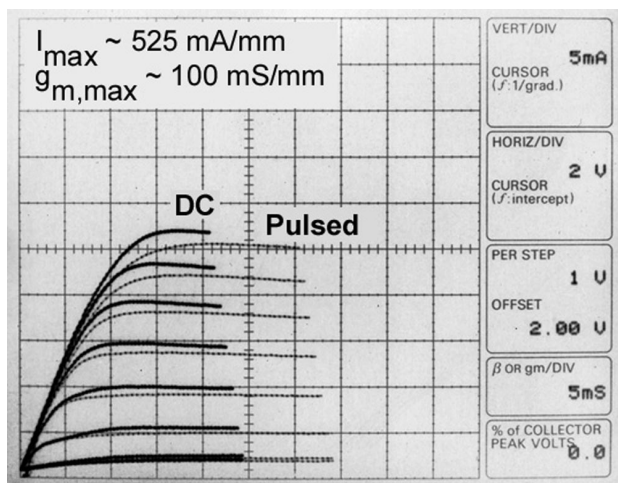
FIG. 5. I - V characteristics for devices fabricated on sample E ( L_g = 1.25 \mu\text{m} , L_{ds} = 3 \mu\text{m} , and w = 50 \mu\text{m} ).
