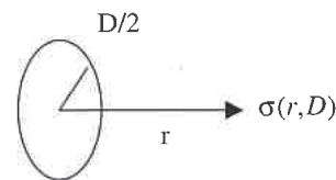
Fig. 10—Stress generated by a finite sized pancake YAG source
