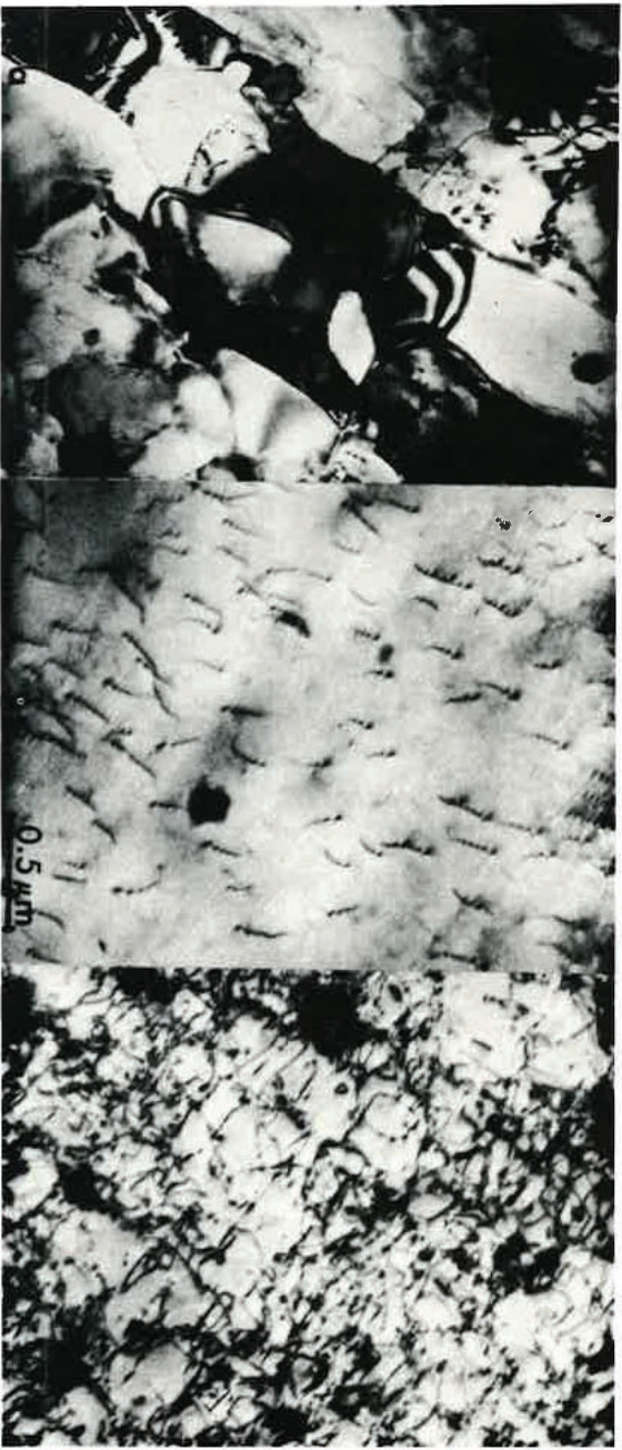
Fig. 5. Microstructure of 5086 H32 aluminum sheet before and after welding and laser shocking. (a) Initial condition - 5086 H 32, (b) After welding - in the heat-affected zone adjacent to the weld zone, and (c) After laser shocking - in the heat-affected zone adjacent to the weld zone.
