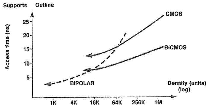
Fig. 8-8 Comparison of speed and density of CMOS, Bipolar and BiCMOS SRAMs. 34 Reprinted with permission of Semiconductor International.
