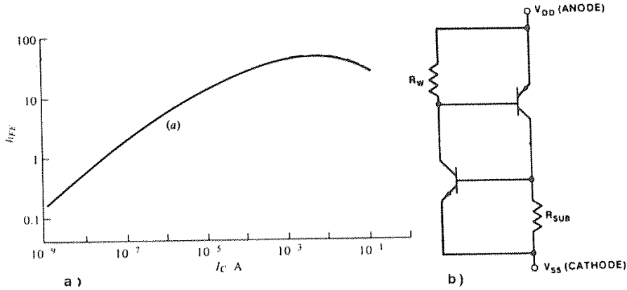
Fig. 6-20 (a) Dependence of current gain on the collector current. (b) Equivalent circuit model of the latchup structure in CMOS, including the parasitic resistances, R_W and R_{SUB} .
