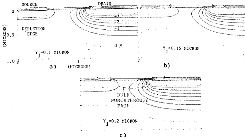
Fig. 6-15 Simulated 2-D potential profile for p -channel MOSFETs with Y_j = 0.1, 0.15 , and 0.2 \mu\text{m} . The drain and gate bias are -3 \text{ V} and 0 \text{ V} , respectively. 22 From K. M. Cham, S.-Y. Oh, D. Chin, and J. L. Moll, Computer-Aided Design and VLSI Device Development , 2nd Ed., Copyright Kluwer Academic, 1989. Reprinted with permission.
