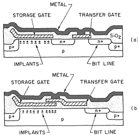
Fig. 8-14 High-capacity (Hi-C) dynamic RAM structure with arsenic (+) and deeper boron (-) implants. (a) One-transistor cell with single-level polysilicon. (b) Double-level polysilicon cell. 35 (© 1978 IEEE).
