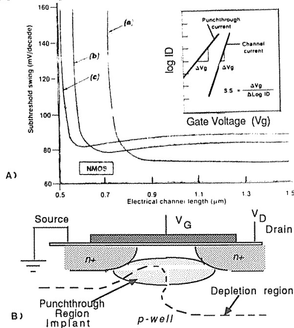
Fig. 5-24 (A) Subthreshold slope versus electrical channel length for NMOS devices ( V_{Tn} = 0.7 \text{ V} ), having a common threshold adjustment implant and punchthrough implant doses of: of: (a) zero; (b) 2 \times 10^{11} \text{ cm}^{-2} ; and (c) 3 \times 10^{11} \text{ cm}^{-2} . 27 Reprinted with permission of Semiconductor International. (B) NMOS cross-section with implant placed into punchthrough region.
