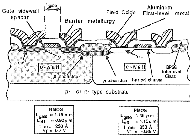
Fig. 6-10 Cross section of a twin-well 1.2- \mu m CMOS structure. 12 Reprinted with permission of Semiconductor International.
