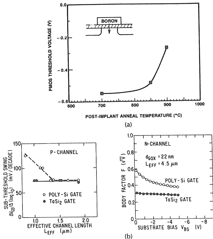
Fig. 6-17 (a) Boron penetration through the gate oxide causes the threshold voltage in BF 2 -implanted PMOS devices to shift positive at anneal temperatures above \sim 800^{\circ}\text{C} . 123 (© 1989 IEEE). (b) Sub-threshold characteristics versus effective channel length for poly-gate and TaSi 2 -gate PMOS devices. 118 (© 1984 IEEE).
