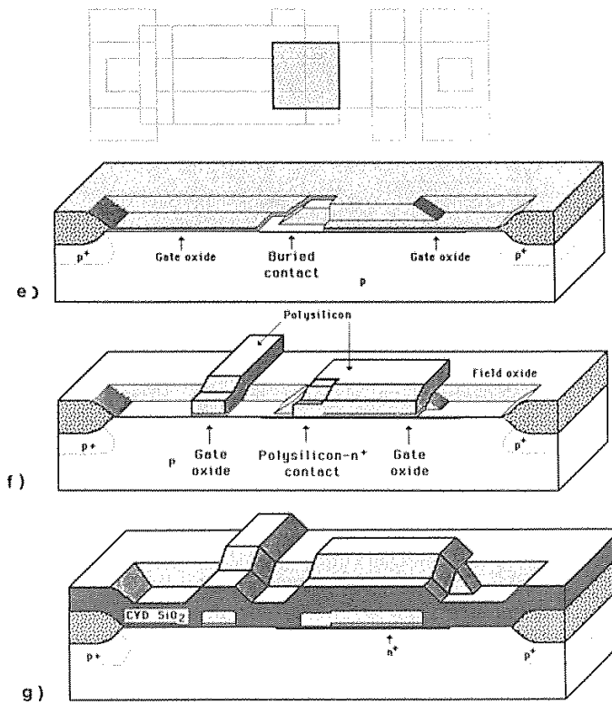
Fig. 5-15 (e) Buried contact etching. (f) Patterning of the polysilicon layer followed by gate oxide etching. (g) Deposition of the CVD SiO 2 layer followed by the diffusion of the drain and source regions. From Maly, Atlas of IC Technologies .
