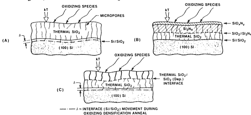
Fig. 6-37 Effects of oxidizing densification anneal: (a) \text{SiO}_2 films; (b) \text{SiO}_2 - \text{Si}_3\text{N}_4 dual dielectric; (c) thermal \text{SiO}_2 - deposited \text{SiO}_2 multilayered stacked films. 76 (© 1988 IEEE).
