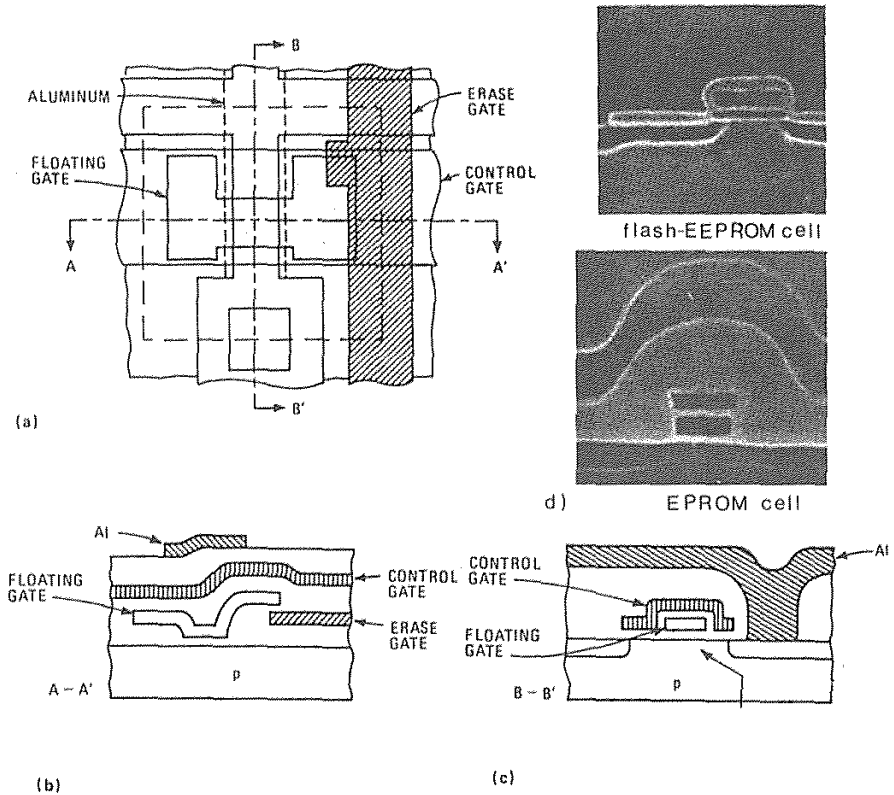
Fig. 8-40 Triple-poly flash-EEPROM cell from Toshiba: (a) Layout; (b) Cross section of the cell; (c) Section at right angles to the section shown in part (b); 101 (d) SEM pictures of double-poly flash-EEPROM and EPROM cells. 99 (© 1988 IEEE).
