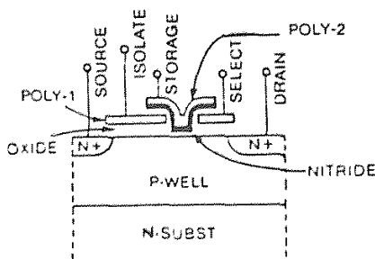
Fig. 8-37. Cross-sectional structure of an MNOS memory cell. 107 (© 1983 IEEE).
