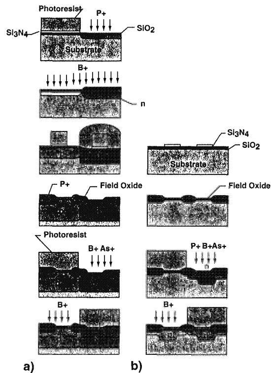
Fig. 5-4 Fabrication sequences for: a) conventional-diffused-well and; b) high-energy-implanted-well processes.
