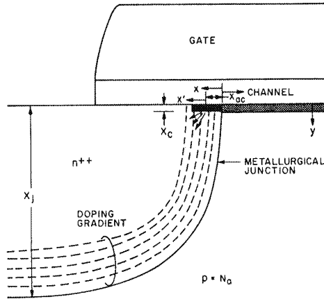
Fig. 5-15 Details of structures near the vicinity of the channel end. The dotted lines are contours of constant concentration. Dark region represents the accumulation layer. 21 (© 1987 IEEE).
