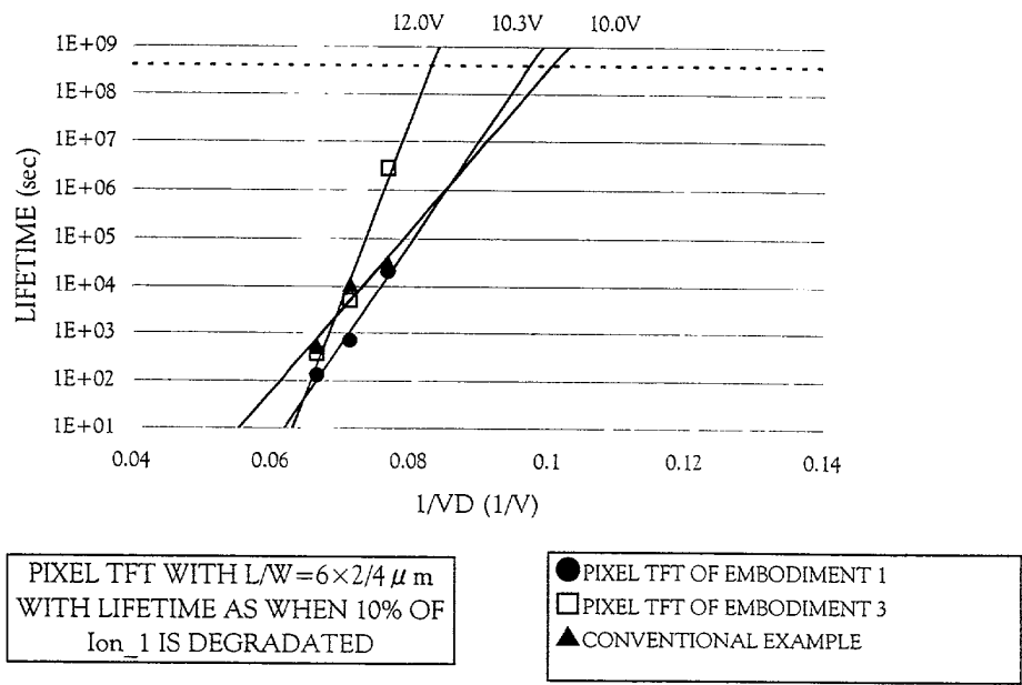
FIG. 20 MEASUREMENT RESULT OF 10-YEAR GUARANTEE
