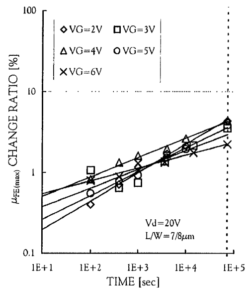
CHARACTERISTICS CHANGE OF N-CHANNEL TFT UNDER TRANSIENT STRESS
