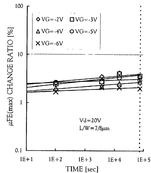
CHARACTERISTICS CHANGE OF P-CHANNEL TFT UNDER TRANSIENT STRESS
