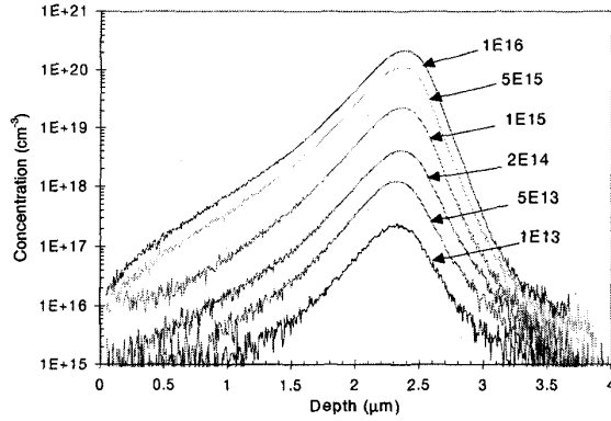
Fig. 4. As-implanted profiles of phosphorus implants at an energy of 3.0 MeV, a 5° tilt, and a 17° rotation.
