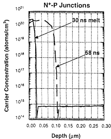
Fig. 9-19 Spreading resistance profile (SRP) for a phosphorus doped P-GILD formed in a p -type doped substrate. Note that x_j increases with surface melt time and the diffusion profile forms a "box" type profile with no anomalous tail. 53
