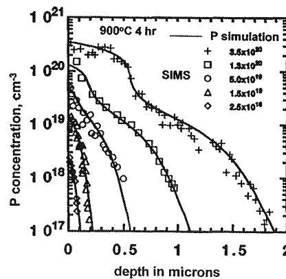
Fig. 9-10 Phosphorus diffusion profile for several surface concentrations. Note the presence of the "kink" and "tail" regions only for the high concentration diffusions. Excellent agreement exists between simulated and measured (SIMS) profiles. 68 Courtesy of American Physical Society.
