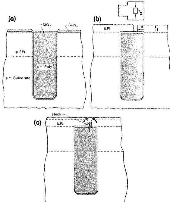
Fig. 8-25 Key processing steps of the SEOT technology. 71 (© 1988 IEEE).
