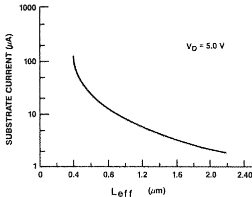
Fig. 5-28 The maximum substrate current due to impact ionization produced at a drain voltage of 5 V vs effective channel length for 250\text{Å} gate oxide transistors. 34 (© 1986 IEEE).
