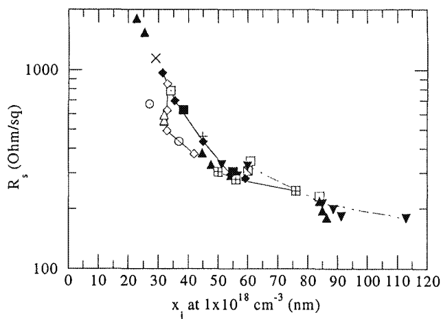
Fig. 5-22 Comparison of p -type sheet-resistance and junction-depth data for spike-anneals using various implant-and-annealing conditions. The data set includes a 400^\circ\text{C}/\text{sec} ramp-up-rate and 0.2\text{-keV} implant-energy. Note that all the data points fall in a rather narrow band. No one has been able to make a 30\text{-nm} junction with a 300\text{-}\Omega/\text{sq} sheet-resistance using ion-implantation and conventional rapid-thermal-annealing. 32
