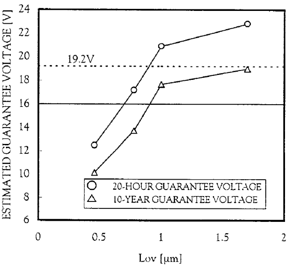
FIG. 31 DEPENDENCE ON L_{ov} LENGTH OF ESTIMATED GUARANTEE VOLTAGE (10% OF ON CURRENT IS DEGRADATED) ( L_g/W = 10/8 \mu\text{m} )
