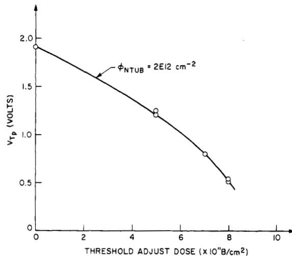
Fig. 3 Sensitivity of the p-channel transistor threshold to n-tub dose and threshold adjust dose.
