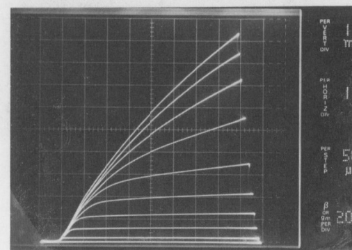
Figure 8. Gate Triggered (p-well) SCR Characteristic for Connection 1 on the RCA CD4007A for Various Values of Lifetime in the npn Base Region (High Injection Level).
