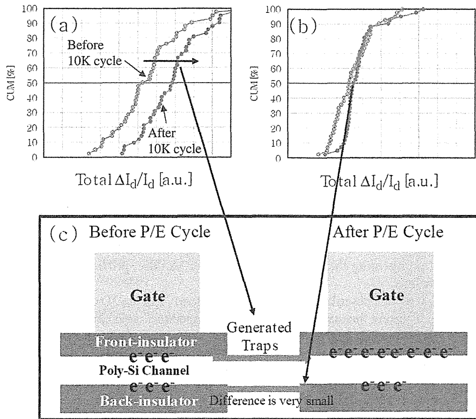
FIGURE 8.41 The RTN distributions before and after 10K P/E cycles at (a) V_{th} = -2 V, (b) V_{th} = 4.5 V. (c) The location differences of traps before and after 10K P/E cycle. Traps were generated between poly-Si and front-insulator by P/E cycling.
