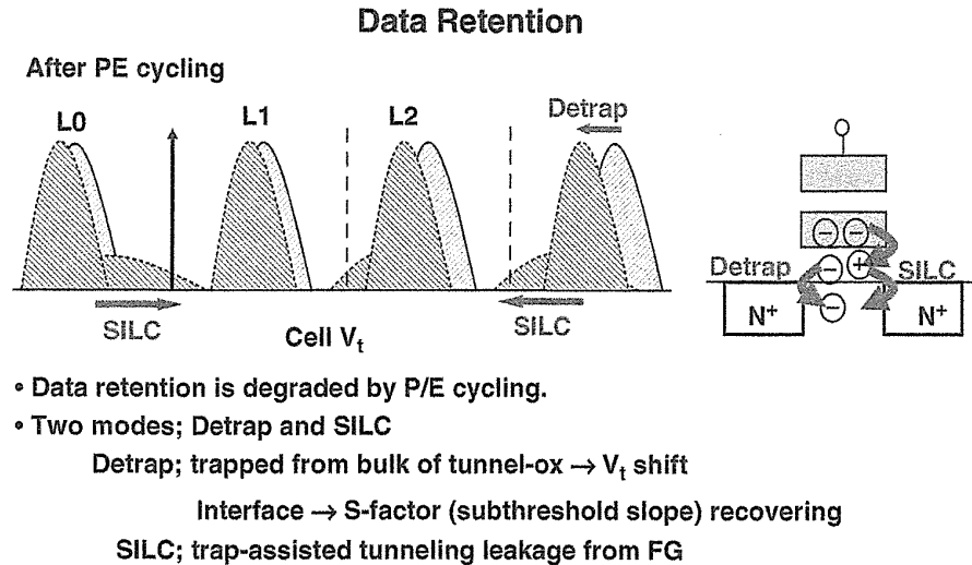
FIGURE 6.2 Data retention phenomena.
