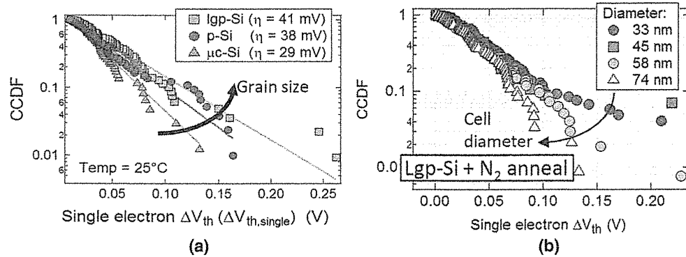
FIGURE 8.27 (a) Complementary cumulative distributions (CCDF = 1-CDF) of threshold voltage shifts \Delta V_{th, \text{single}} caused by single electron trapping (see Fig. 8.25) for different poly-Si materials. CCDFs follow an exponential distribution with the average values \eta given in the inset. (b) A weak reduction of the impact per trap on the \Delta V_{th, \text{single}} is observed by increasing the cell diameter.
