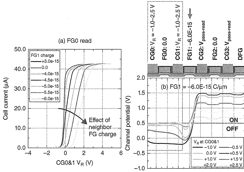
FIGURE 7.73 (a) Cell I_d - V_g of FG0 read under various FG1 charge. (b) Channel potential at FG1 = -6.0E-15 C/μm. When FG1 has a negative charge, the transconductance is degraded due to increasing channel resistance under FG1.
