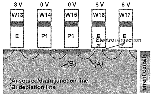
FIGURE 6.65 Device simulation is performed on the BV_{dss} measurement condition at PP1 pattern. Current density shows the punch-through of WL15 off-cell at V_{bl} = 4 \text{ V} . DIBL (drain-induced barrier lowering) generates punch-through between source and drain in unselected cell. Electrons generated by punch-through are injected at nearby cells (disturb happens). Lower V_t cell shows larger DIBL.
