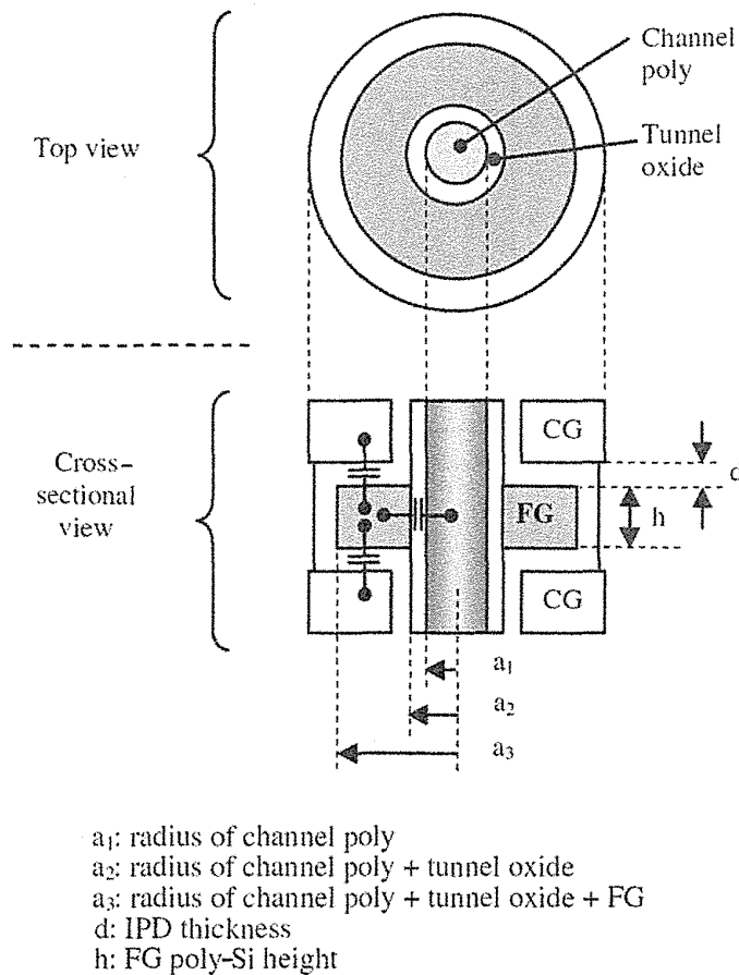
FIGURE 7.58 Floating-gate capacitance of the DC-SF cell.
