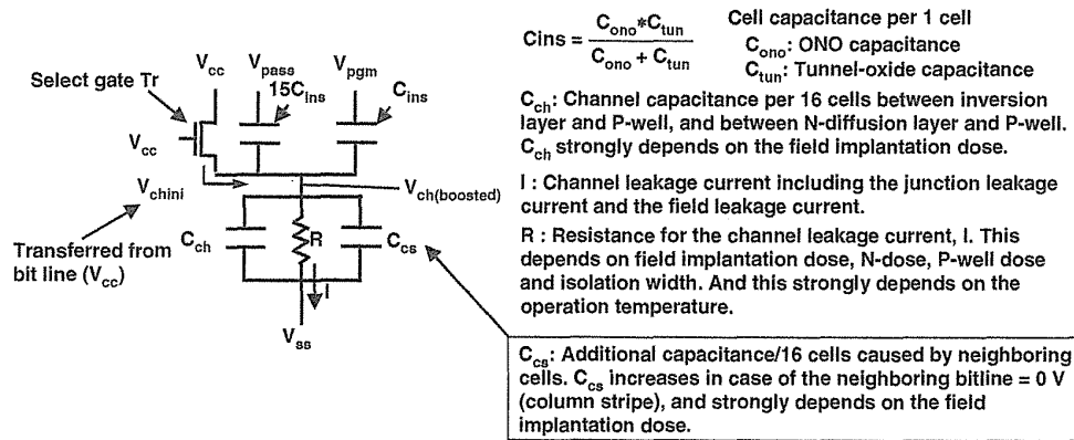
FIGURE 6.53 The equivalent circuit for self-boosting model, including an additional capacitor, C_{cs} . In the column stripe pattern, C_{cs} becomes large and decreases the channel voltage, V_{ch} . As a result, the number of programmable cycles (NOP) is limited by the column stripe pattern.
