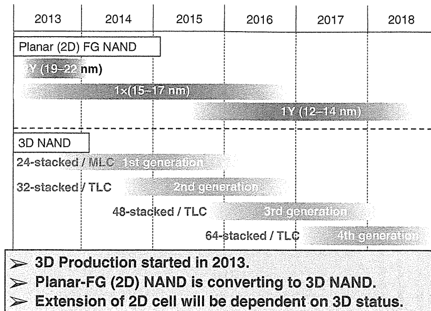
FIGURE 8.52 Transition from a planar 2D NAND cell to a 3D NAND cell.
