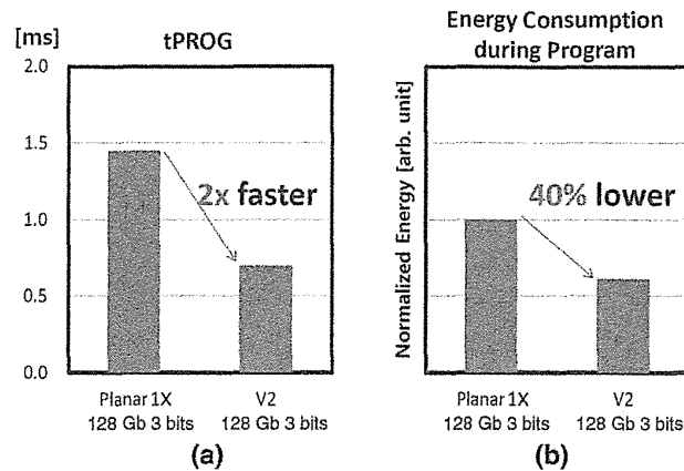
FIGURE 7.41 The program time and energy consumption during programming. Program time could be improved 200% ( \times 2 ), and energy consumption can be reduced 40%.
