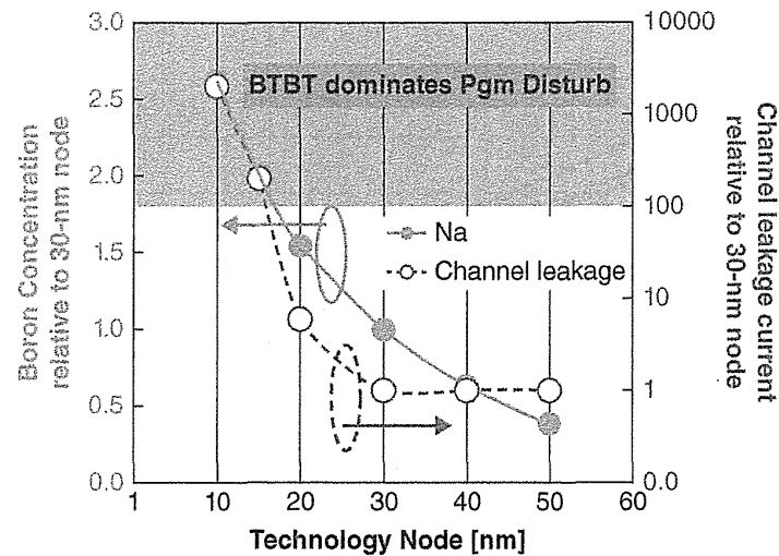
FIGURE 6.59 Technology scaling trend. Channel boron concentration is determined to maintain a charge-neutral V_i across technology nodes. At the sub-20-nm node, BTBT current becomes the dominant mechanism for NAND-cell program disturb.
