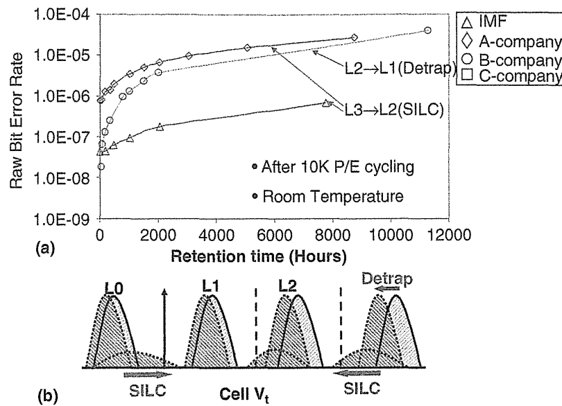
FIGURE 6.29 RBER versus room-temperature retention time following 10K P/E cycles. RBER increases as retention time.
