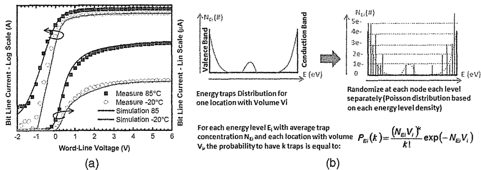
FIGURE 8.33 (a) Measured and simulated cell current at -20^\circ\text{C} and 85^\circ\text{C} (linear and logarithmic scale). The measured cell is in the median of the array distribution. (b) RTF modeling strategy. The model assumes a poisson distribution from the traps density concentration used for calibrating of (a). No other parameters need to be assumed.
