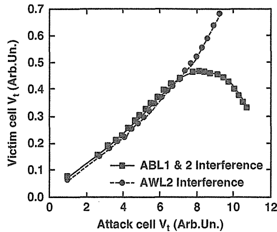
FIGURE 6.74 Victim cell V_t shift versus attack cell programmed V_t . Negative V_t shift phenomena are observed in the case of attack ABL1 and ABL2. Victim cell V_t is corresponding to L1 for MLC.
