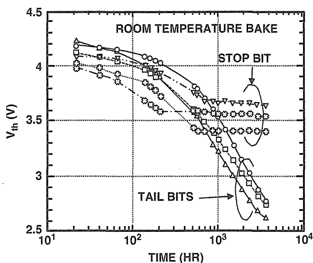
FIGURE 6.27 Charge loss characteristics of the anomalous cells of “stop bit.” There are three bits whose rapid charge loss is suddenly and randomly stopped.
