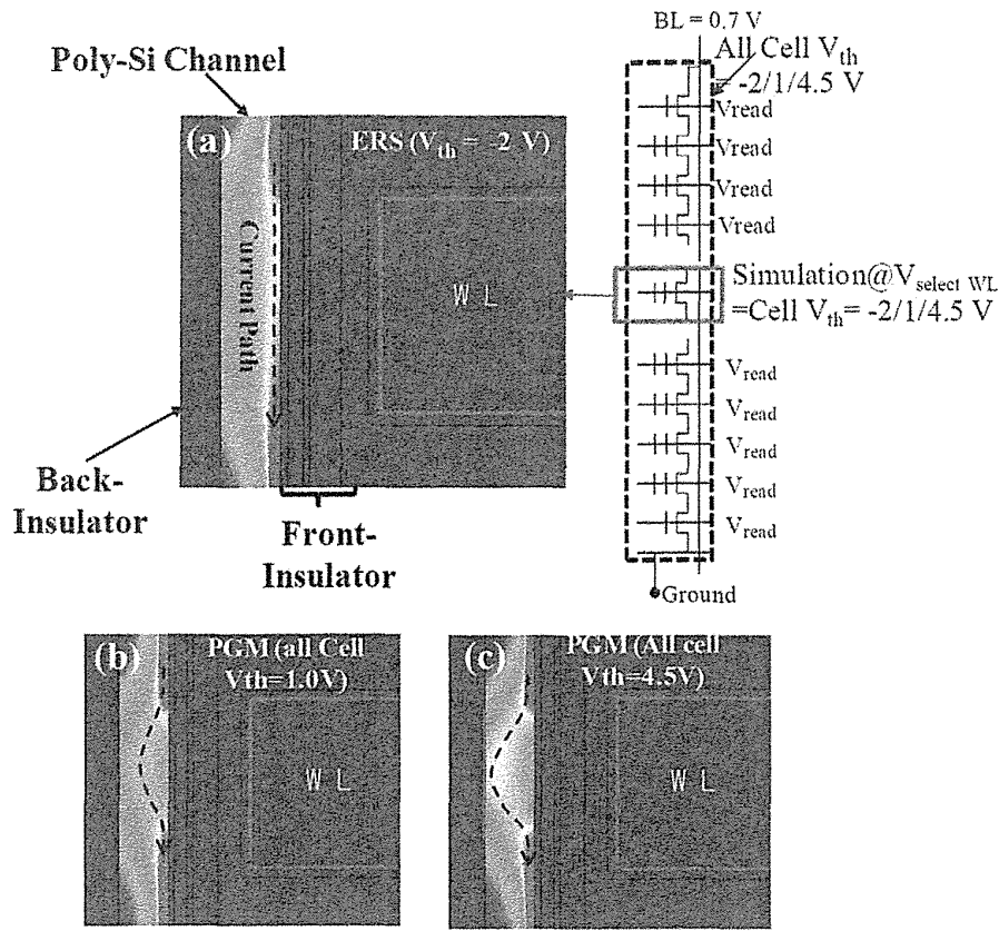
FIGURE 8.37 The simulation results for current path of select WL in V-NAND for (a) V_{select WL} = \text{cell } V_{th} = -2 V, (b) V_{select WL} = \text{cell } V_{th} = 1 V, and (c) V_{select WL} = \text{cell } V_{th} = 4.5 V, respectively.
