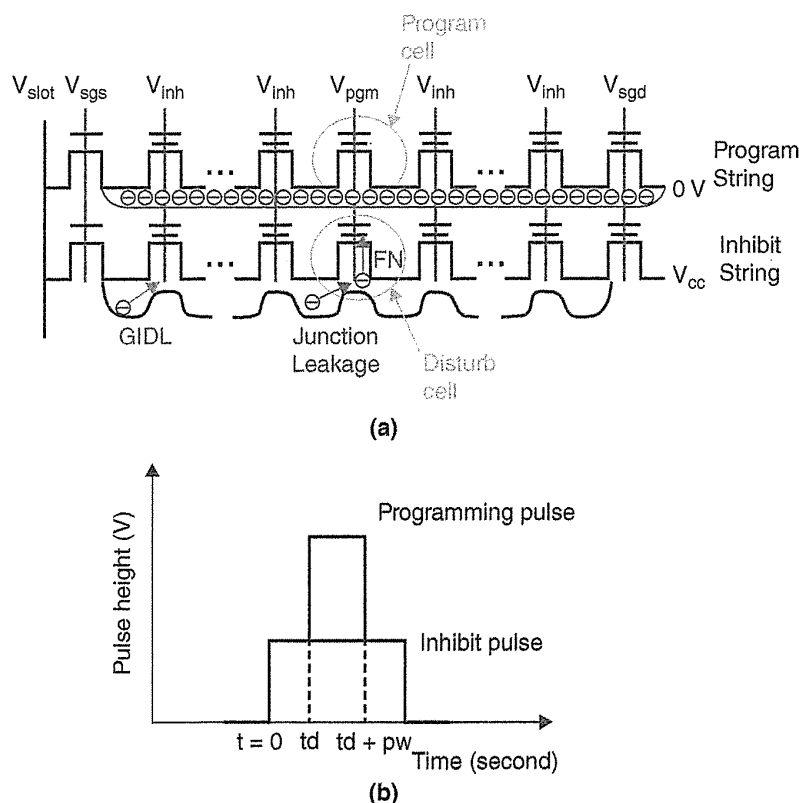
FIGURE 6.57 (a) Bias conditions of NAND strings during programming, along with the different program disturb mechanisms. (b) Program and inhibit-pulse waveforms. A td is a ramp-up delay between inhibit pulse ( V_{inh} ) and programming pulse ( V_{pgm} ).
