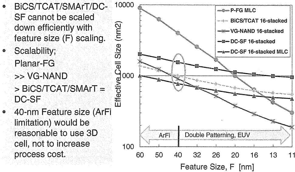
FIGURE 8.4 Scalability of 3D NAND flash memory cell.
