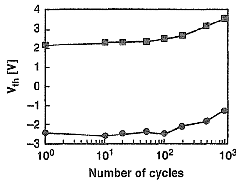
FIGURE 7.84 Program/erase cycling endurance characteristics of the DC-SF cell.
