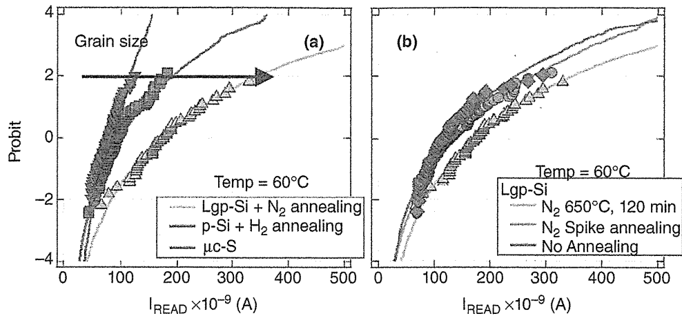
FIGURE 8.28 (a) The highest I_{\text{READ}} values are registered for lgp-Si. Interestingly, at low percentiles, the predicted currents converge. (b) Long \text{N}_2 annealing slightly shifts the reading current at higher values.
