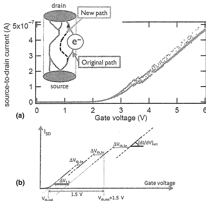
FIGURE 8.25 (a) A selected example of a I_{SD} - V_G characteristic measured with V_D = 0.1 V and 1-mV resolution (6000 dots are individual measurement points). This example clearly shows how the curve consists of a discrete number of well-defined curves, each corresponding to a different configuration of percolation paths from source to drain. Trapping of individual electrons (partially) blocks a conduction path as schematically drawn in the inset. A net negative charging is observed with increasing V_G . (b) Schematic reproduction of the I_{SD} - V_G characteristic in (a) with definitions. (i) \Delta V_{th,1e} is the V_{th} shift caused by the trapping of one electron. Three different shifts are indicated. (ii) (dI/dV)_{act} is the transconductance of the linear parts of the curve. (iii) \Delta V_{1.5} is the total V_{th} -shift between the V_G = V_{th,init} and V_G = V_{th,init} + 1.5 V. It is a measure of the charging component in the I_{SD} - V_G curve.
