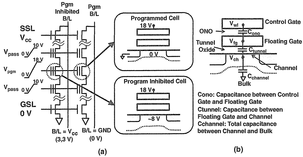
FIGURE 6.52 Self-booted program inhibit voltage generation. (a) Bias conditions for self-booting. (b) Capacitance model for coupling ratio calculation.
