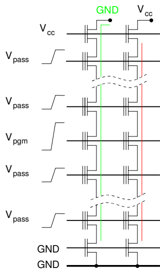
Figure 31. NAND array bias condition during program, highlighting the self-boosting effect.
