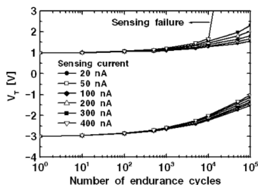
Figure 3. Endurance characteristics of a NAND cell [63], © 2004 IEEE.
