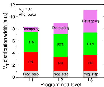
Figure 28. Contributions to the width of the V_T distribution after cycling and bake for different programmed levels [239], © 2015 IEEE.
