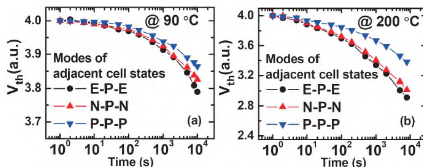
Figure 37. Charge retention characteristics for a charge-trap based 3D NAND as a function of the state of the adjacent cells and for different temperatures [305], © 2015 IEEE.
