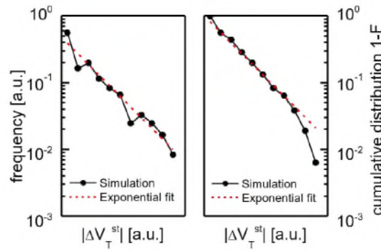
Figure 6. Probability density function ( left ) and cumulative distribution ( right ) for the threshold voltage shift determined by the charging of a single interfacial trap, \Delta V_T^1 , in a decananometer NAND Flash cell [112], © 2008 IEEE.
