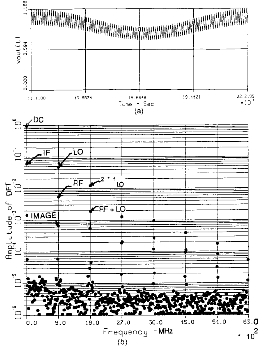
Figure 4. Output voltage of the resistively matched mixer: (a) time domain; (b) frequency domain.
