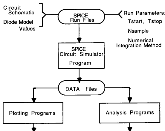
Figure 1. Flowchart of the program.
