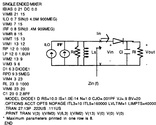
Figure 3. Resistively matched single-ended mixer: circuit diagram and corresponding SPICE run file.
