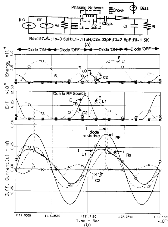
Figure 9. Optimized mixer when C_{j0} = .25\text{pF} ; (a) circuit diagram; (b) energy pattern and differential currents.
