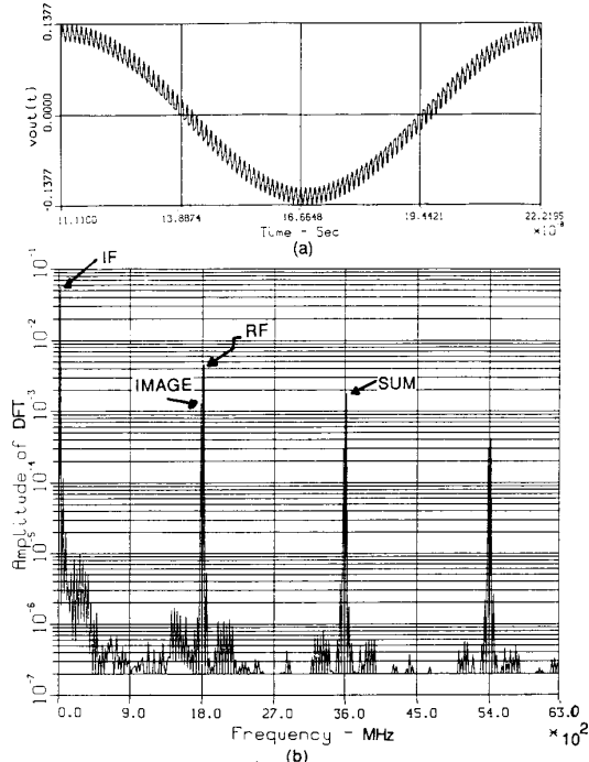
Figure 7. Output v_{out} of the resistively matched balanced mixer: (a) time domain; (b) frequency domain.
