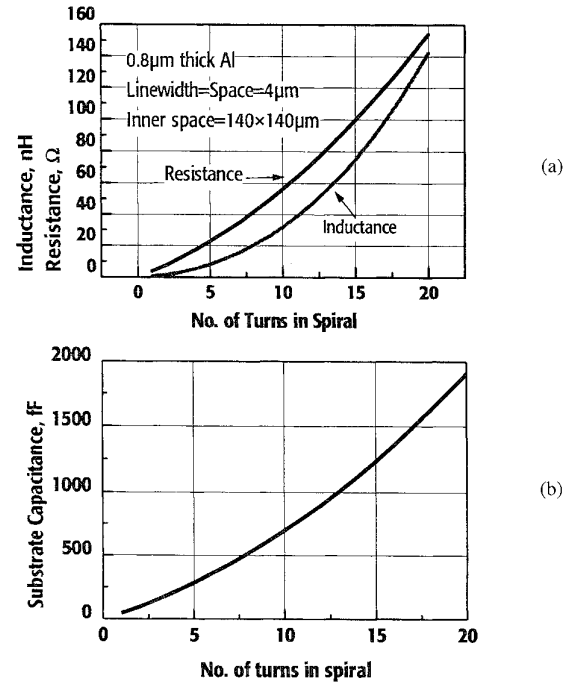
Fig. 5. Design curves for square spiral on-chip inductor. (a) Inductance and resistance of spiral versus number of turns and (b) capacitance of inductor (assuming it is an equipotential) to substrate through 1 \mu\text{m} thick field oxide.
