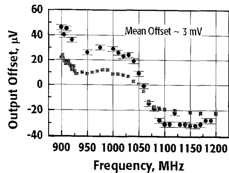
Fig. 15. Change in output dc offset as LO frequency is varied, as measured on two samples of the front-end IC.
