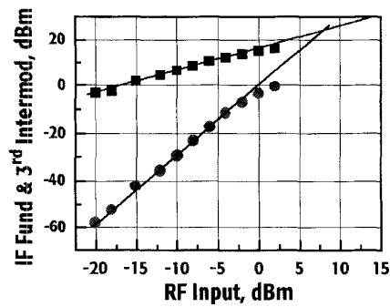
Fig. 12. Linearity of combined LNA and mixer, measured with two-tone input in LNA passband.
