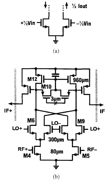
Fig. 8. (a) Linear MOS transconductor. (b) Downconversion mixer circuit diagram.
