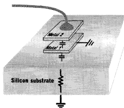
Fig. 10. Structure of RF input pad to LNA. Metal 1 shields the input signal from spreading resistance of substrate.
