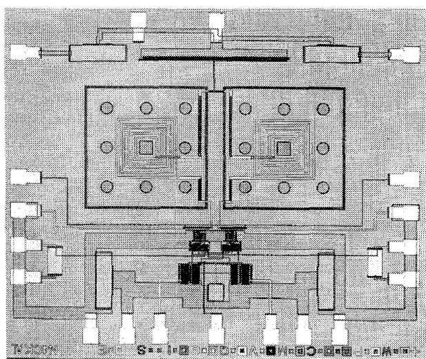
Fig. 9. Die photograph of front-end IC, consisting of LNA and downconversion mixer.
