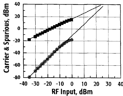
Fig. 14. Second-order intercept plots growth of detected envelope at dc versus AM signal strength. This is of importance in a direct-conversion receiver.
