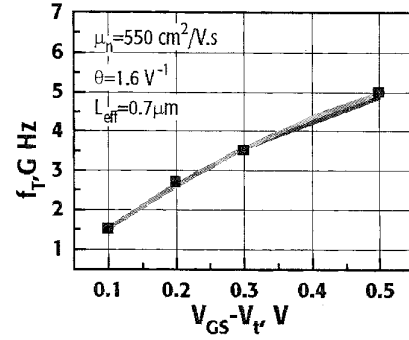
Fig. 4. Measured f_T versus V_{GS} - V_t for MOSIS 1- \mu\text{m} NMOSFET (points) fitted to simple expression (line).
