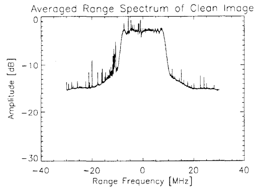
Fig. 4. Averaged Range Spectrum of Cleaned Image
