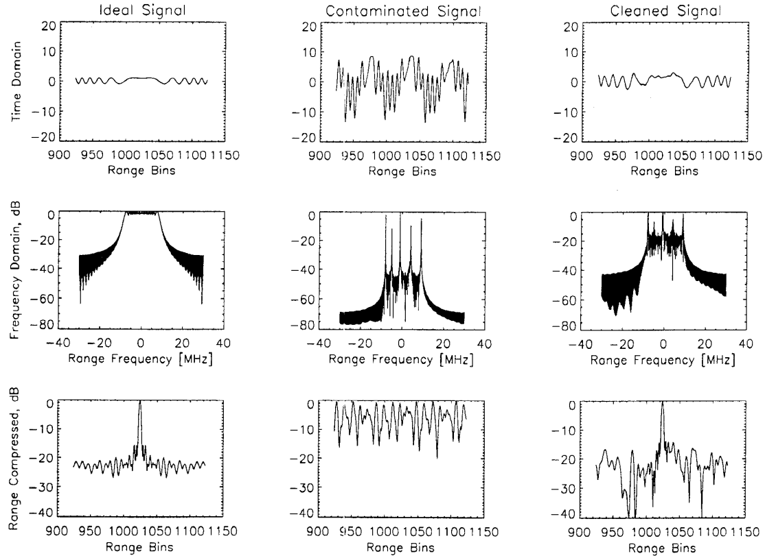
Fig. 2. Simulation results demonstrating the effectiveness of the adaptive filter applied to RF interference suppression. The three columns show the ideal, contaminated and cleaned signal respectively. The first row shows the real part of the signal in the time domain, the second row shows the signal in the frequency domain, and the third row shows the range compressed signal.
