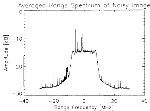
Fig. 3. Averaged Range Spectrum of Noisy Image
