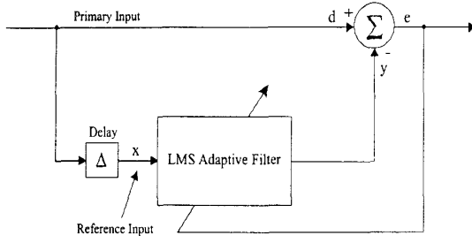
Fig. 1. LMS Adaptive Filter
