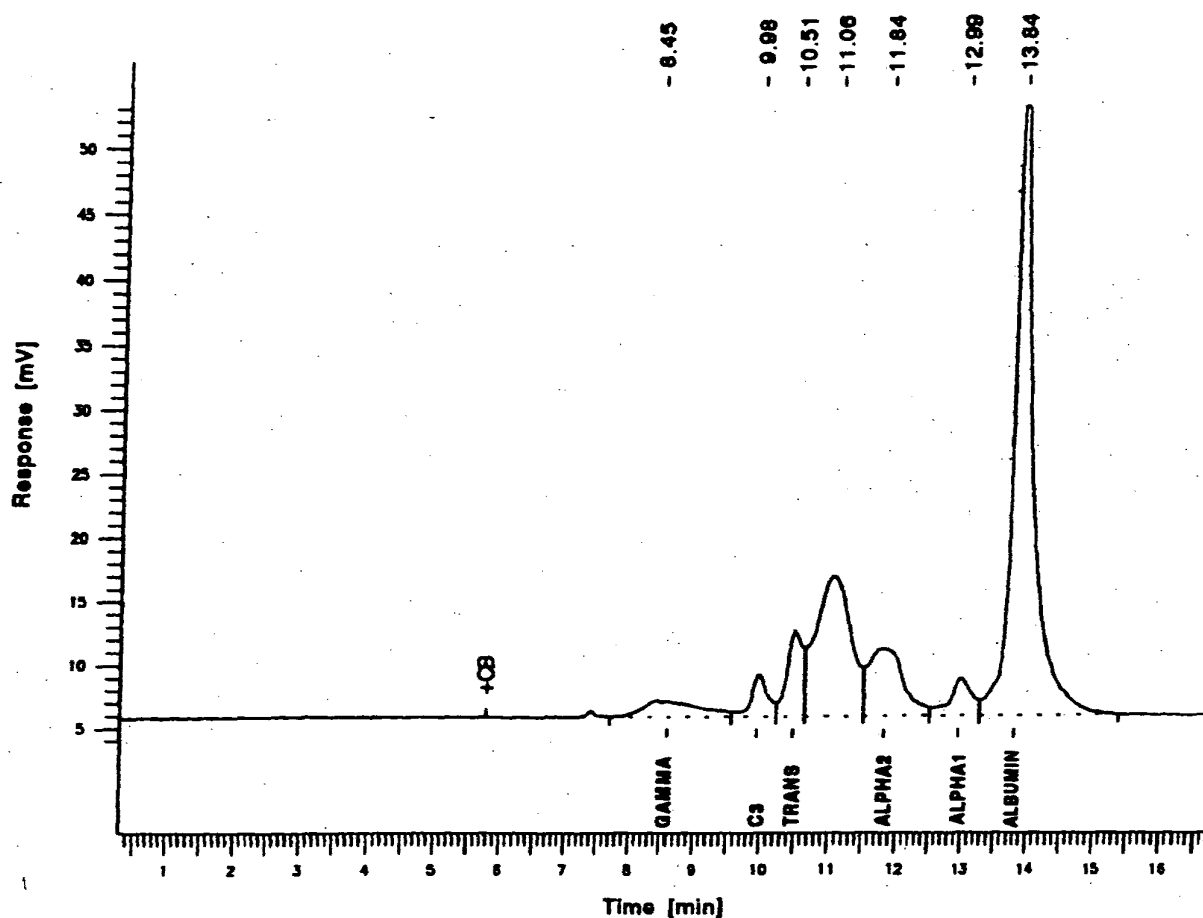
Fig. 1. Electropherogram of a monoclonal IgA detected by capillary electrophoresis showing separation from \alpha_2 and transferrin components. Conditions: Fused-silica capillary, 72 cm \times 50 \mu m I.D.; detection, 200 nm; applied voltage, 18 kV; buffer, 50 mM boric acid, pH 9.7, containing 1 mM calcium lactate.
