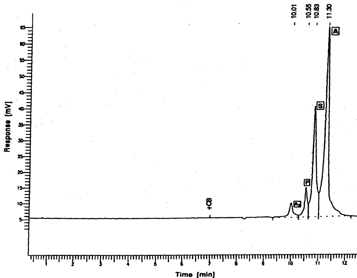
Fig. 3. Electropherogram of a Biorad haemoglobin A 2 control, showing haemoglobin A, S, F and A 2 as marked. Conditions: Applied Biorad system fused-silica capillary, 72 cm × 50 μm I.D.; detection, 200 nm; applied voltage, 15 kV; injection, 1 s; running buffer, 0.1 M boric acid, pH 9.98.
