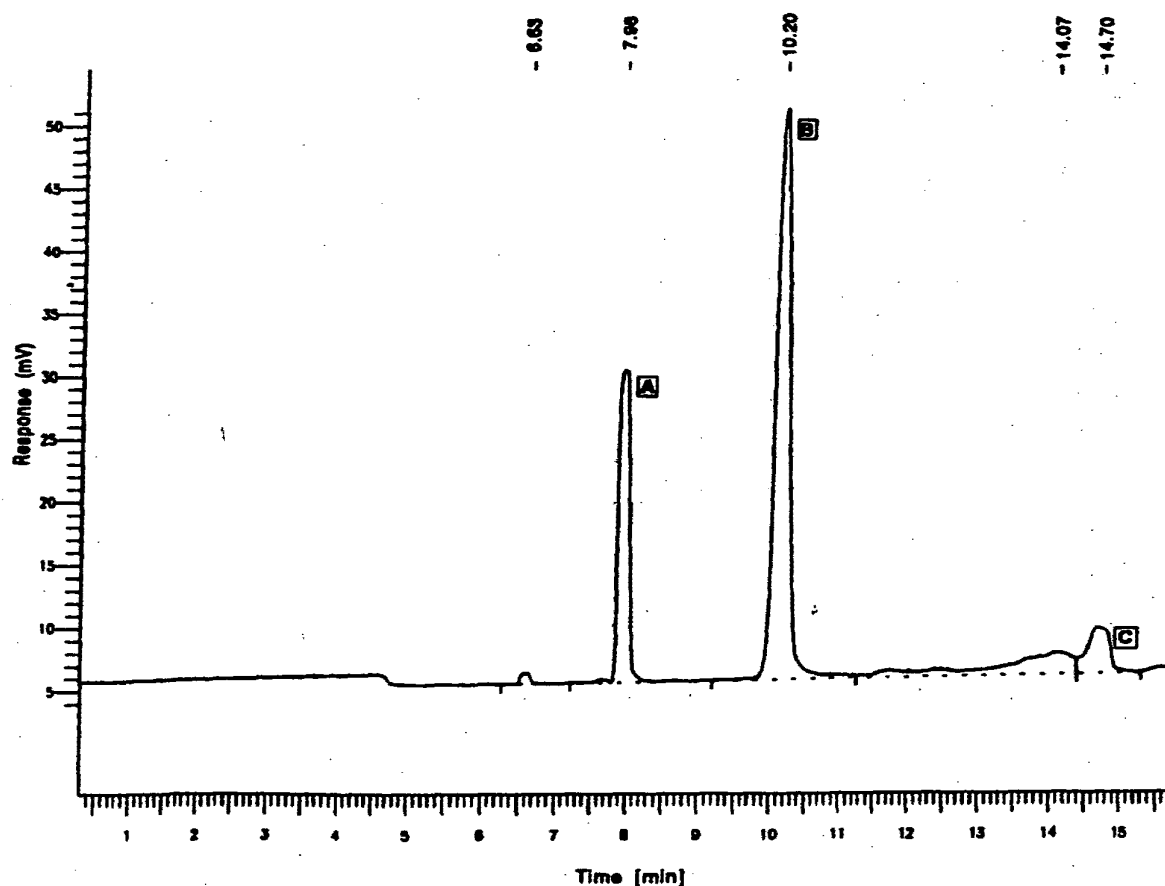
Fig. 2. Electropherogram of human urine proteins showing the components: A = Urea/creatinine; B = Bence Jones protein and C = albumin. Conditions: fused-silica capillary, 72 cm \times 50 \mu m I.D.; detection, 200 nm; applied voltage, 18 kV; running buffer, 150 mM boric acid–1 mM calcium lactate, pH 9.7.
