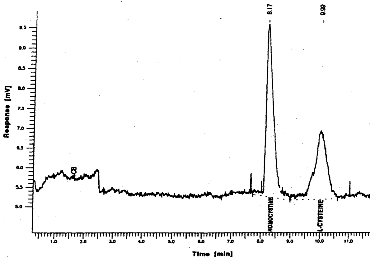
Fig. 4. Electropherogram showing the separation of homocysteine ( 100 \mu\text{M} ) and L-cysteine ( 100 \mu\text{M} ). Conditions: fused-silica capillary, 62 \text{ cm} \times 100 \mu\text{m} I.D.; detection, 200 \text{ nm} ; applied voltage, 15 \text{ kV} ; buffer, 10 \text{ mM} phosphate buffer, \text{pH } 2.5 .
